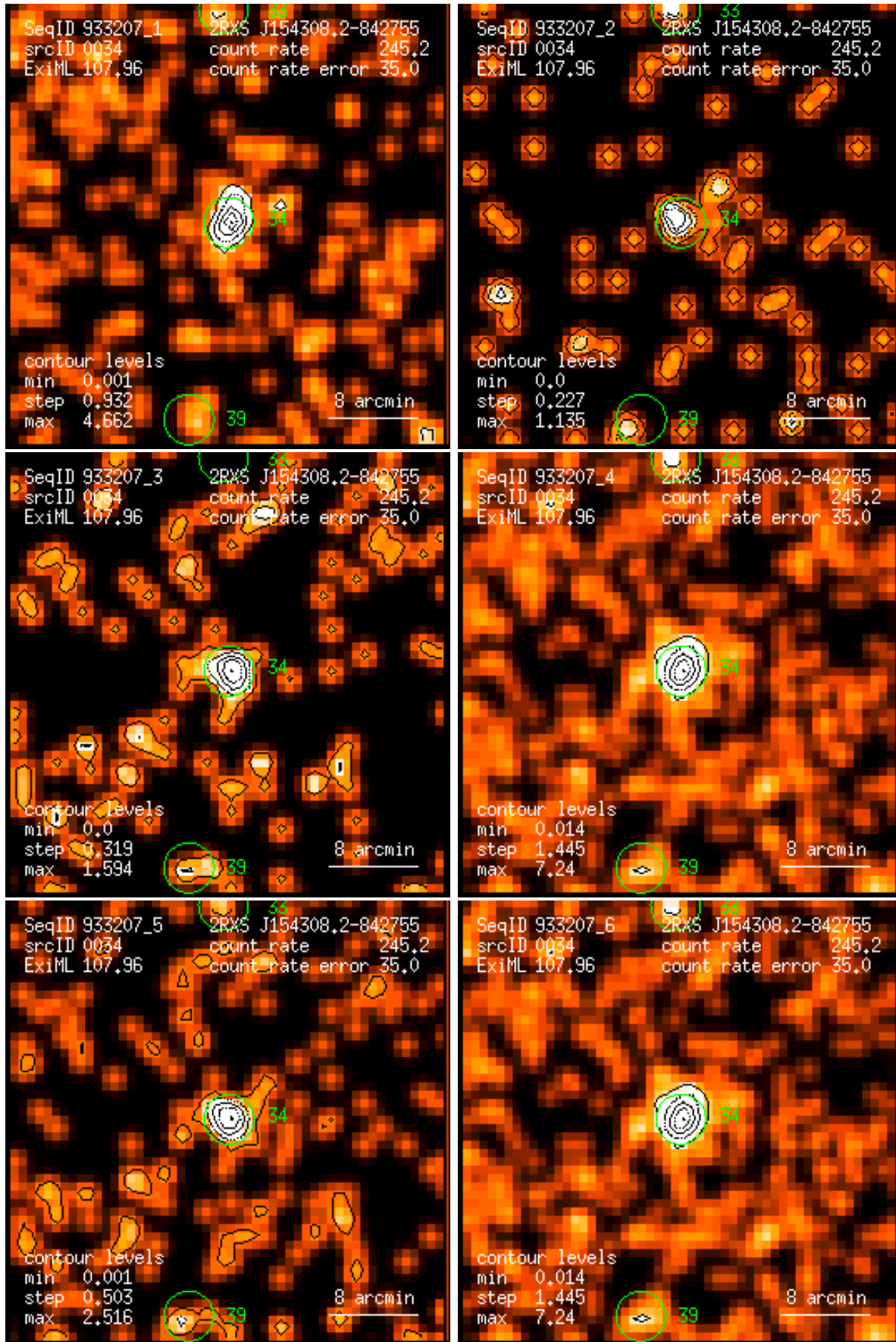
Figure 34: RASS 933207: detection 0034: band rate images, Gaussian filter: (1) PSPC channels 11 – 41, (2) 52 – 90, (3) 91 – 201, (4) 11 – 235, (5) 52 – 201, (6) 11 – 201. Broad band rates in counts/ks. Band rate contour levels in counts/ks/arcmin 2 .
