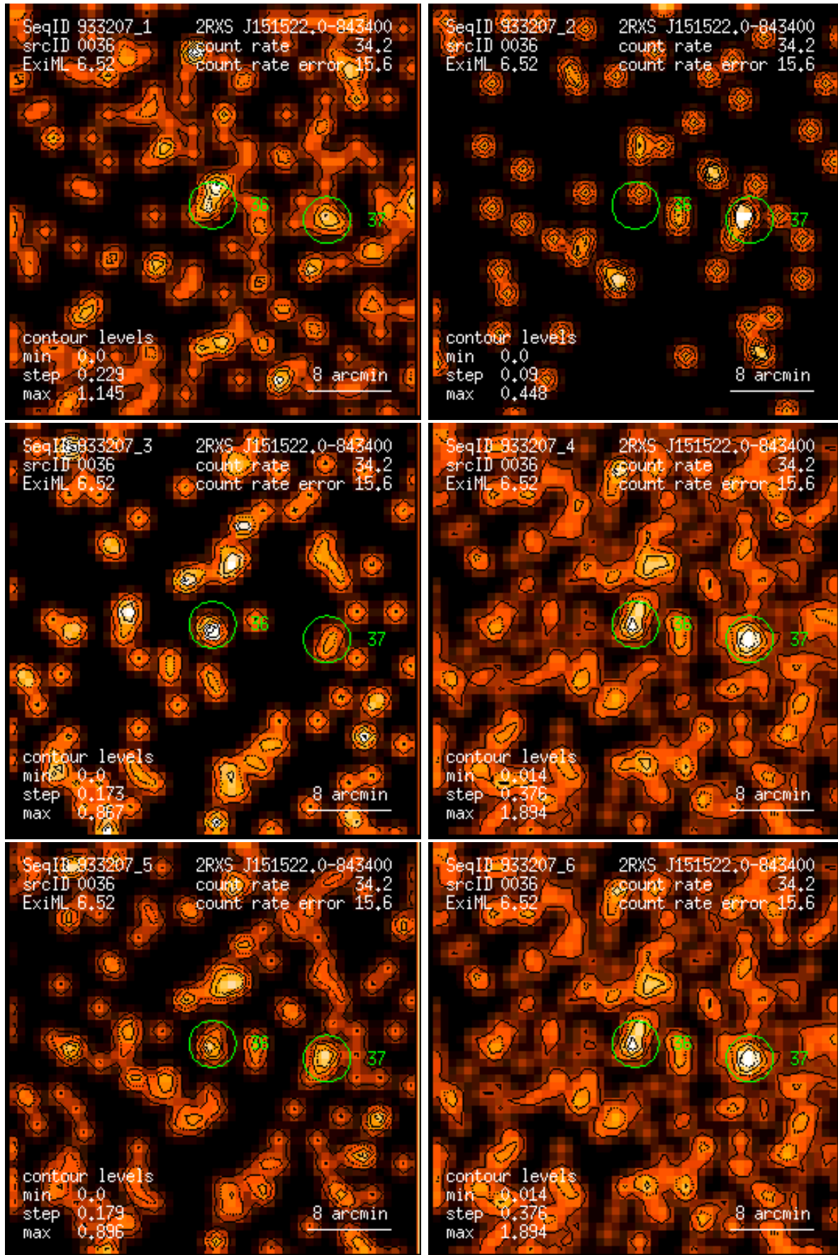
Figure 36: RASS 933207: detection 0036: band rate images, Gaussian filter: (1) PSPC channels 11 – 41, (2) 52 – 90, (3) 91 – 201, (4) 11 – 235, (5) 52 – 201, (6) 11 – 201. Broad band rates in counts/ks. Band rate contour levels in counts/ks/arcmin 2 .
