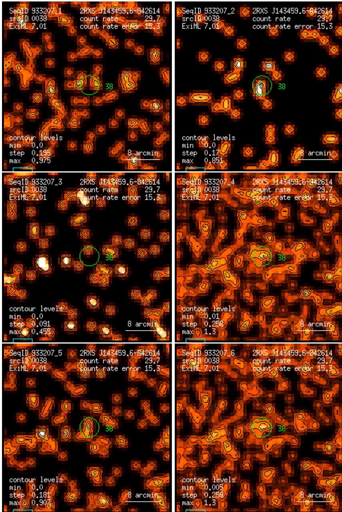
Figure 38: RASS 933207: detection 0038: band rate images, Gaussian filter: (1) PSPC channels 11 – 41, (2) 52 – 90, (3) 91 – 201, (4) 11 – 235, (5) 52 – 201, (6) 11 – 201. Broad band rates in counts/ks. Band rate contour levels in counts/ks/arcmin 2 .
