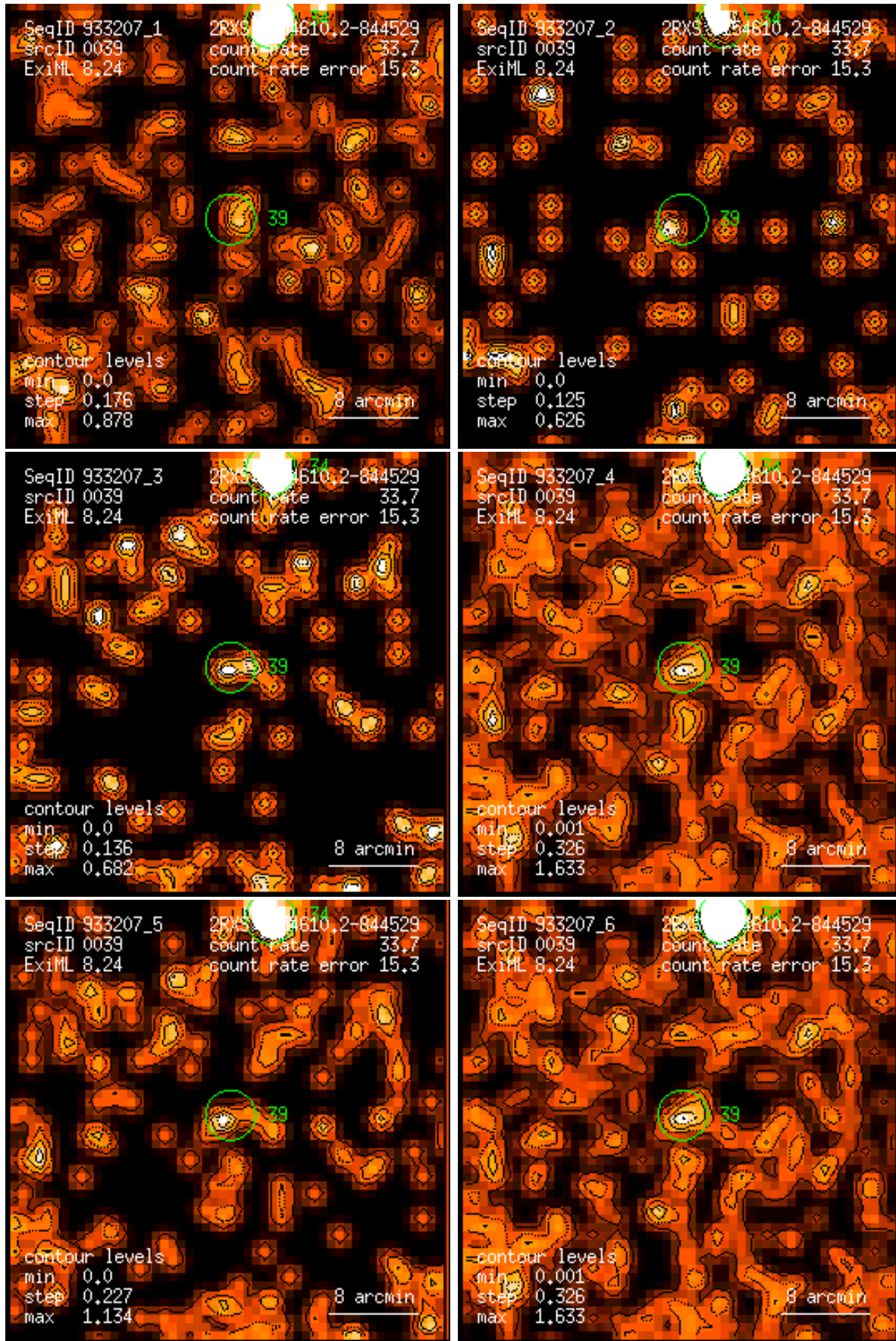
Figure 39: RASS 933207: detection 0039: band rate images, Gaussian filter: (1) PSPC channels 11 – 41, (2) 52 – 90, (3) 91 – 201, (4) 11 – 235, (5) 52 – 201, (6) 11 – 201. Broad band rates in counts/ks. Band rate contour levels in counts/ks/arcmin 2 .
