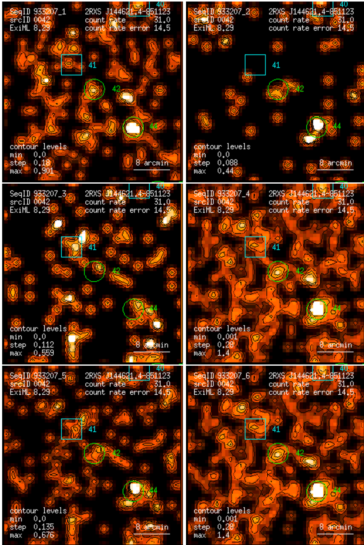
Figure 42: RASS 933207: detection 0042: band rate images, Gaussian filter: (1) PSPC channels 11 – 41, (2) 52 – 90, (3) 91 – 201, (4) 11 – 235, (5) 52 – 201, (6) 11 – 201. Broad band rates in counts/ks. Band rate contour levels in counts/ks/arcmin 2 .
