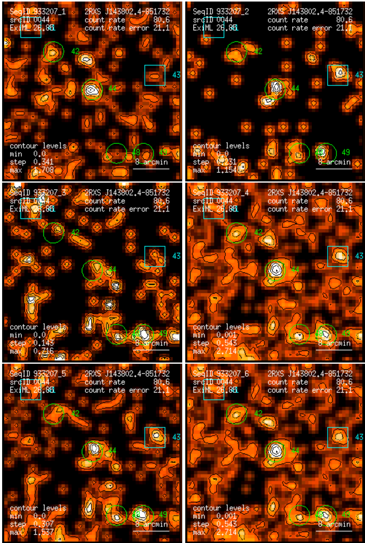
Figure 44: RASS 933207: detection 0044: band rate images, Gaussian filter: (1) PSPC channels 11 – 41, (2) 52 – 90, (3) 91 – 201, (4) 11 – 235, (5) 52 – 201, (6) 11 – 201. Broad band rates in counts/ks. Band rate contour levels in counts/ks/arcmin 2 .
