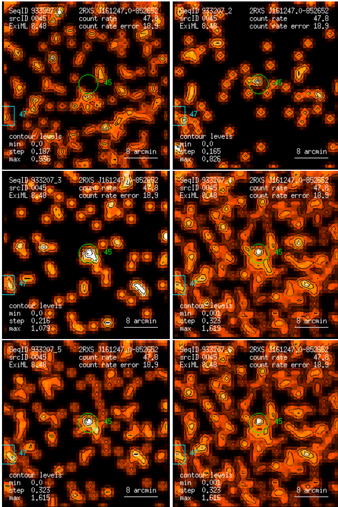
Figure 45: RASS 933207: detection 0045: band rate images, Gaussian filter: (1) PSPC channels 11 – 41, (2) 52 – 90, (3) 91 – 201, (4) 11 – 235, (5) 52 – 201, (6) 11 – 201. Broad band rates in counts/ks. Band rate contour levels in counts/ks/arcmin 2 .
