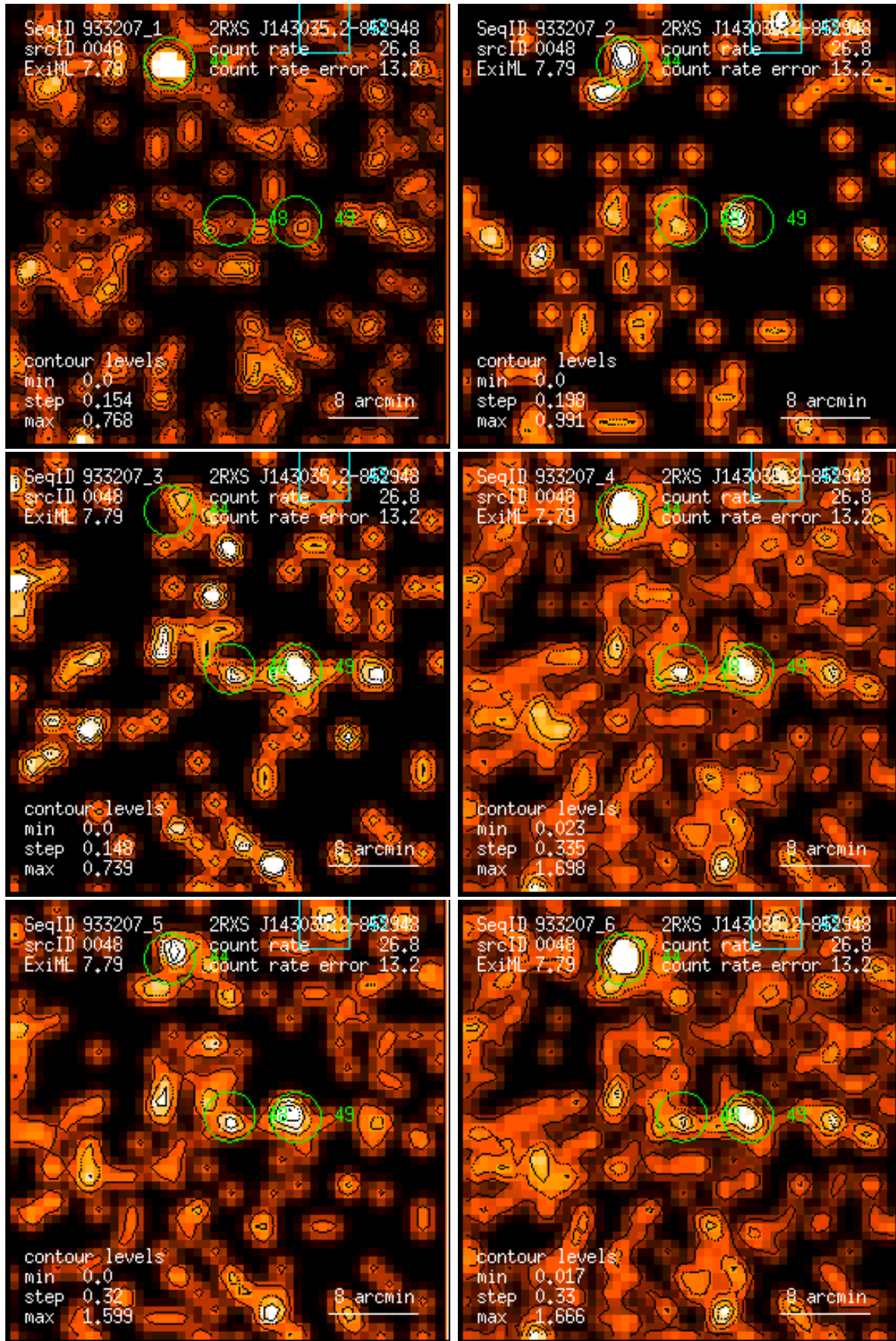
Figure 48: RASS 933207: detection 0048: band rate images, Gaussian filter: (1) PSPC channels 11 – 41, (2) 52 – 90, (3) 91 – 201, (4) 11 – 235, (5) 52 – 201, (6) 11 – 201. Broad band rates in counts/ks. Band rate contour levels in counts/ks/arcmin 2 .
