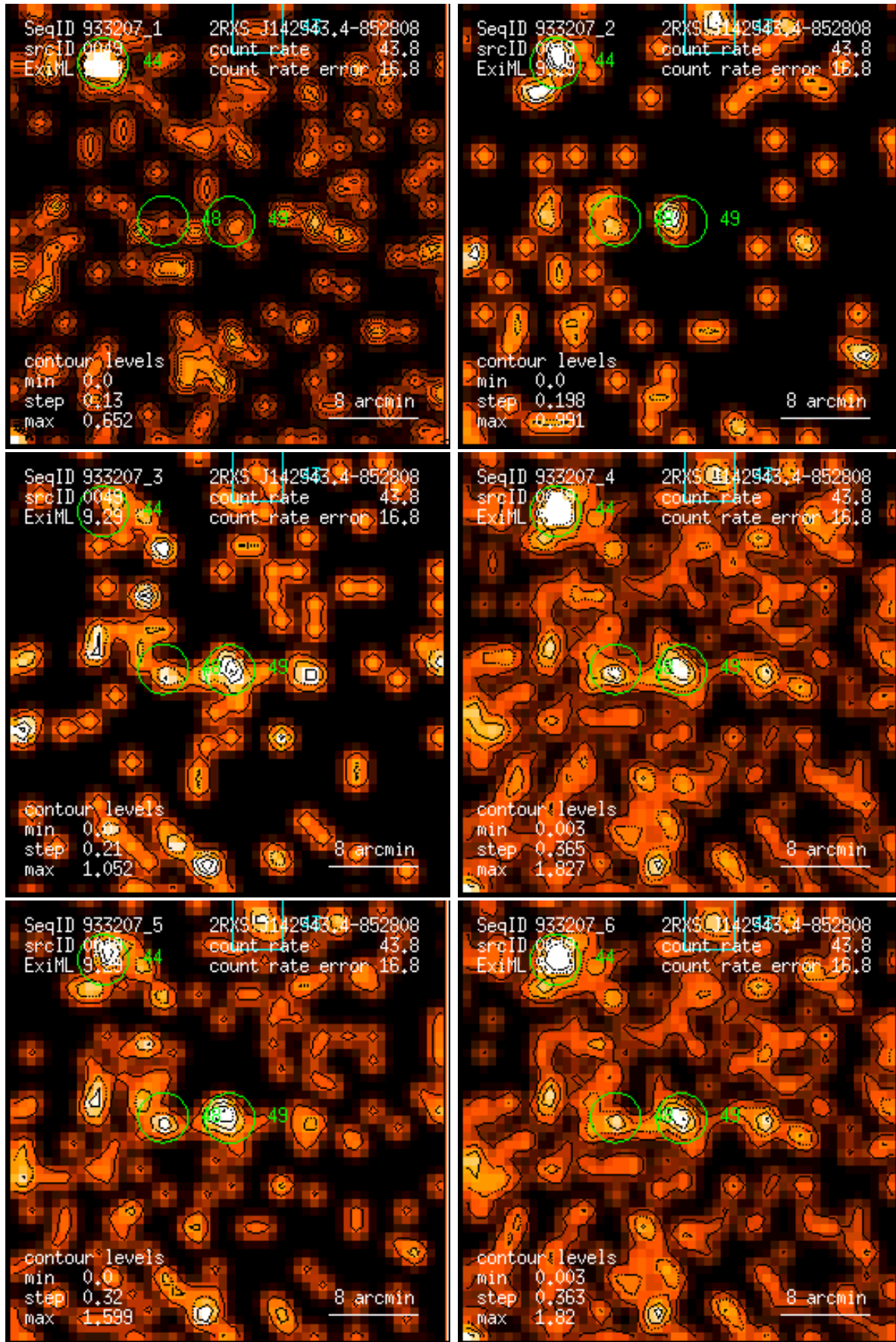
Figure 49: RASS 933207: detection 0049: band rate images, Gaussian filter: (1) PSPC channels 11 – 41, (2) 52 – 90, (3) 91 – 201, (4) 11 – 235, (5) 52 – 201, (6) 11 – 201. Broad band rates in counts/ks. Band rate contour levels in counts/ks/arcmin 2 .
