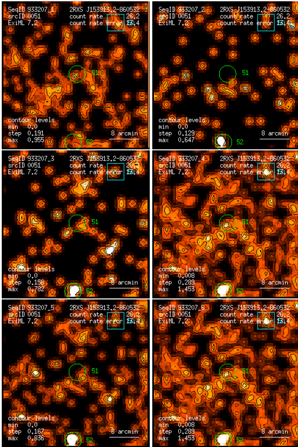
Figure 51: RASS 933207: detection 0051: band rate images, Gaussian filter: (1) PSPC channels 11 – 41, (2) 52 – 90, (3) 91 – 201, (4) 11 – 235, (5) 52 – 201, (6) 11 – 201. Broad band rates in counts/ks. Band rate contour levels in counts/ks/arcmin 2 .
