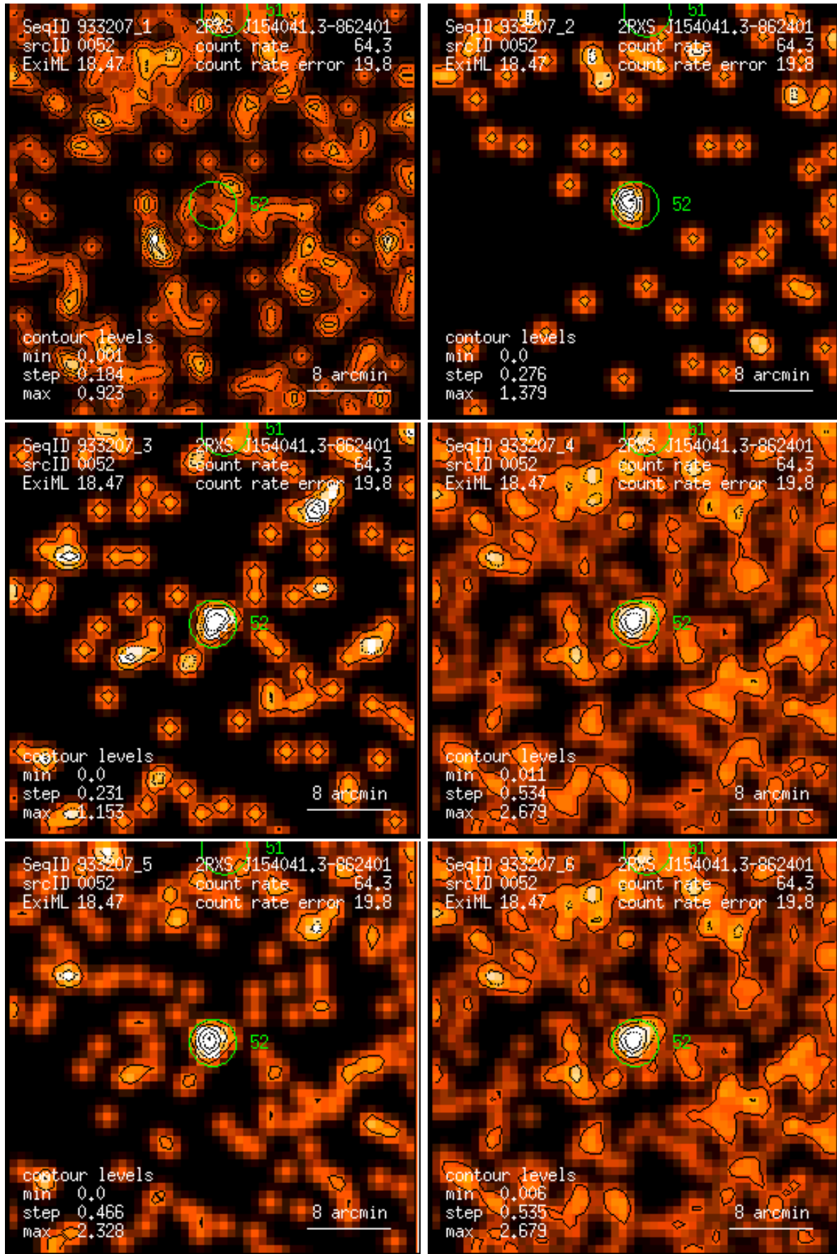
Figure 52: RASS 933207: detection 0052: band rate images, Gaussian filter: (1) PSPC channels 11 – 41, (2) 52 – 90, (3) 91 – 201, (4) 11 – 235, (5) 52 – 201, (6) 11 – 201. Broad band rates in counts/ks. Band rate contour levels in counts/ks/arcmin 2 .
