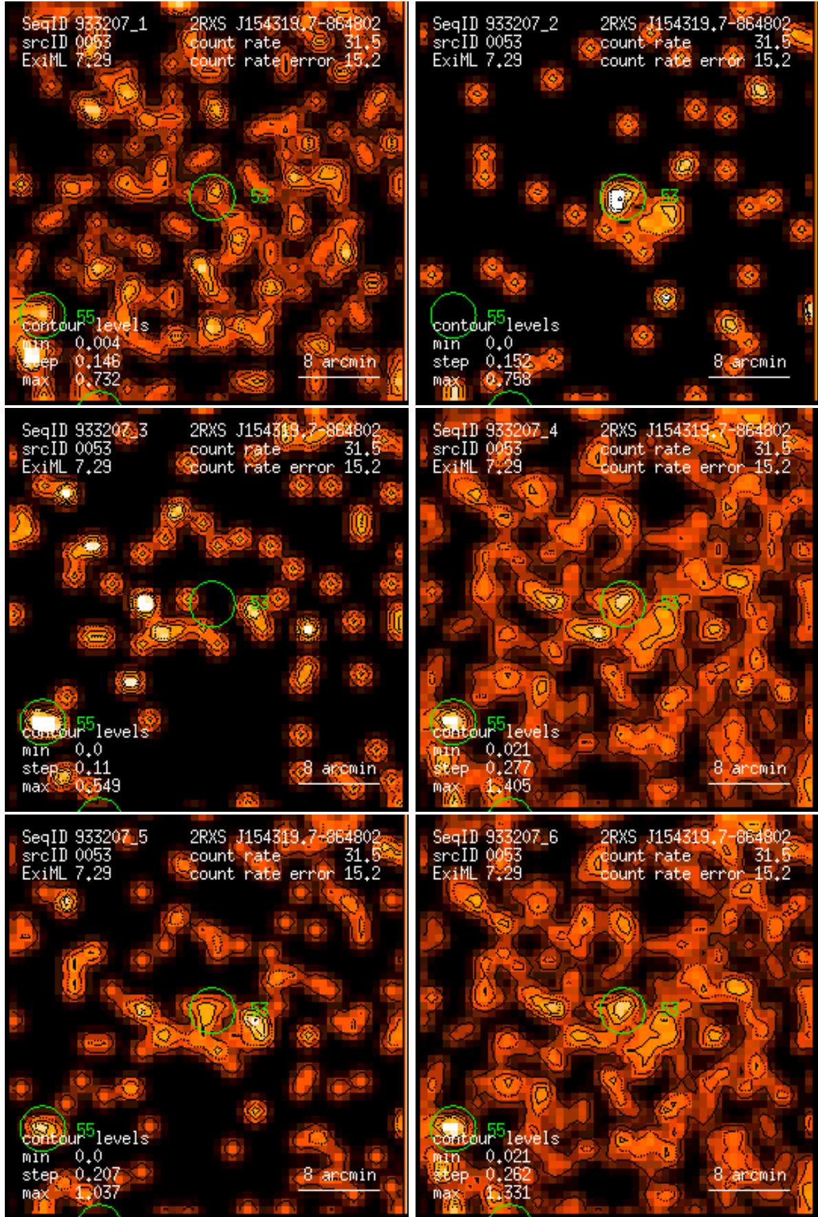
Figure 53: RASS 933207: detection 0053: band rate images, Gaussian filter: (1) PSPC channels 11 – 41, (2) 52 – 90, (3) 91 – 201, (4) 11 – 235, (5) 52 – 201, (6) 11 – 201. Broad band rates in counts/ks. Band rate contour levels in counts/ks/arcmin 2 .
