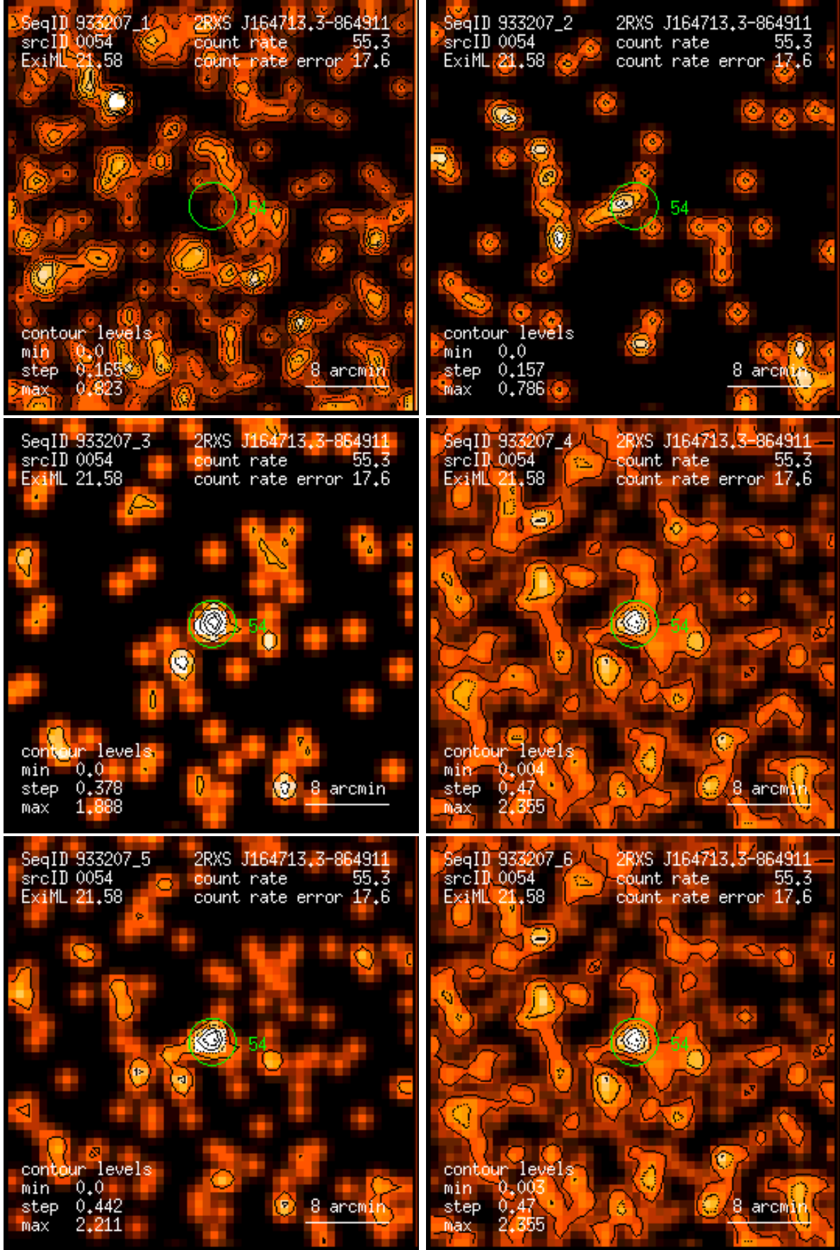
Figure 54: RASS 933207: detection 0054: band rate images, Gaussian filter: (1) PSPC channels 11 – 41, (2) 52 – 90, (3) 91 – 201, (4) 11 – 235, (5) 52 – 201, (6) 11 – 201. Broad band rates in counts/ks. Band rate contour levels in counts/ks/arcmin 2 .
