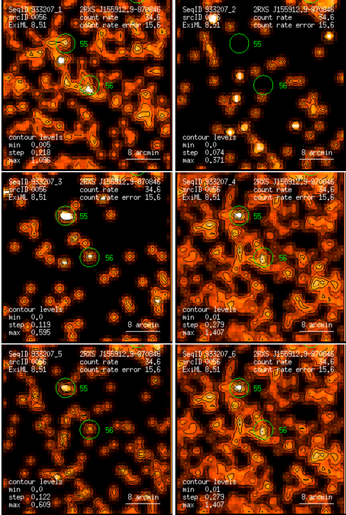
Figure 56: RASS 933207: detection 0056: band rate images, Gaussian filter: (1) PSPC channels 11 – 41, (2) 52 – 90, (3) 91 – 201, (4) 11 – 235, (5) 52 – 201, (6) 11 – 201. Broad band rates in counts/ks. Band rate contour levels in counts/ks/arcmin 2 .
