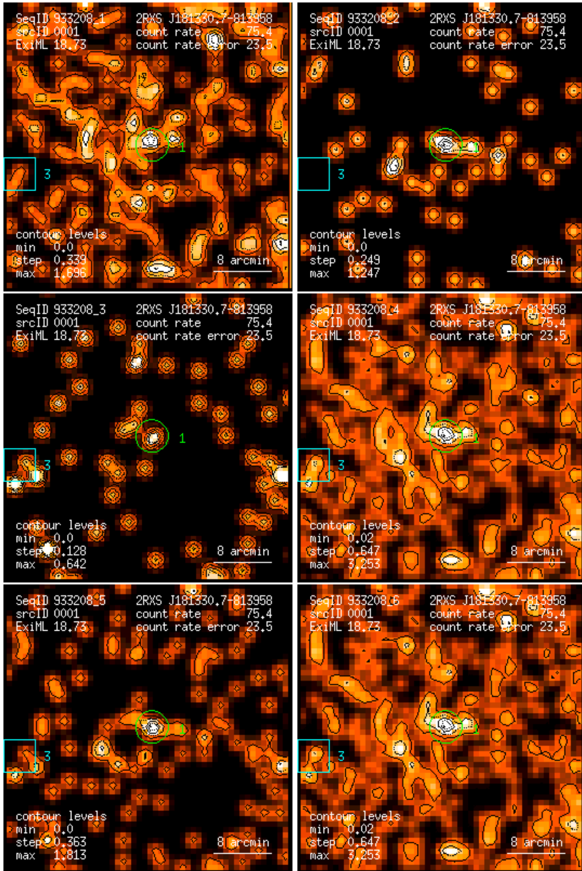
Figure 1: RASS 933208: detection 0001: band rate images, Gaussian filter: (1) PSPC channels 11 – 41, (2) 52 – 90, (3) 91 – 201, (4) 11 – 235, (5) 52 – 201, (6) 11 – 201. Broad band rates in counts/ks. Band rate contour levels in counts/ks/arcmin 2 .
