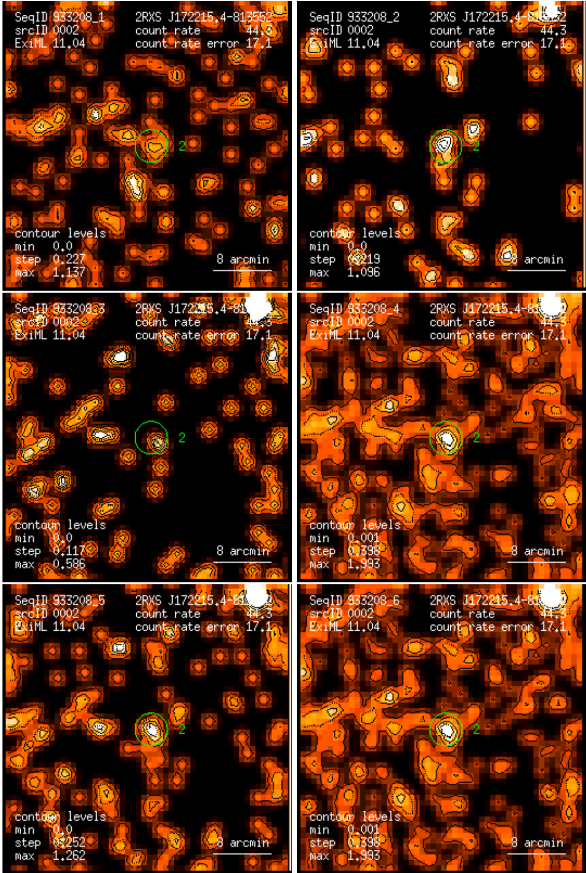
Figure 2: RASS 933208: detection 0002: band rate images, Gaussian filter: (1) PSPC channels 11 – 41, (2) 52 – 90, (3) 91 – 201, (4) 11 – 235, (5) 52 – 201, (6) 11 – 201. Broad band rates in counts/ks. Band rate contour levels in counts/ks/arcmin 2 .
