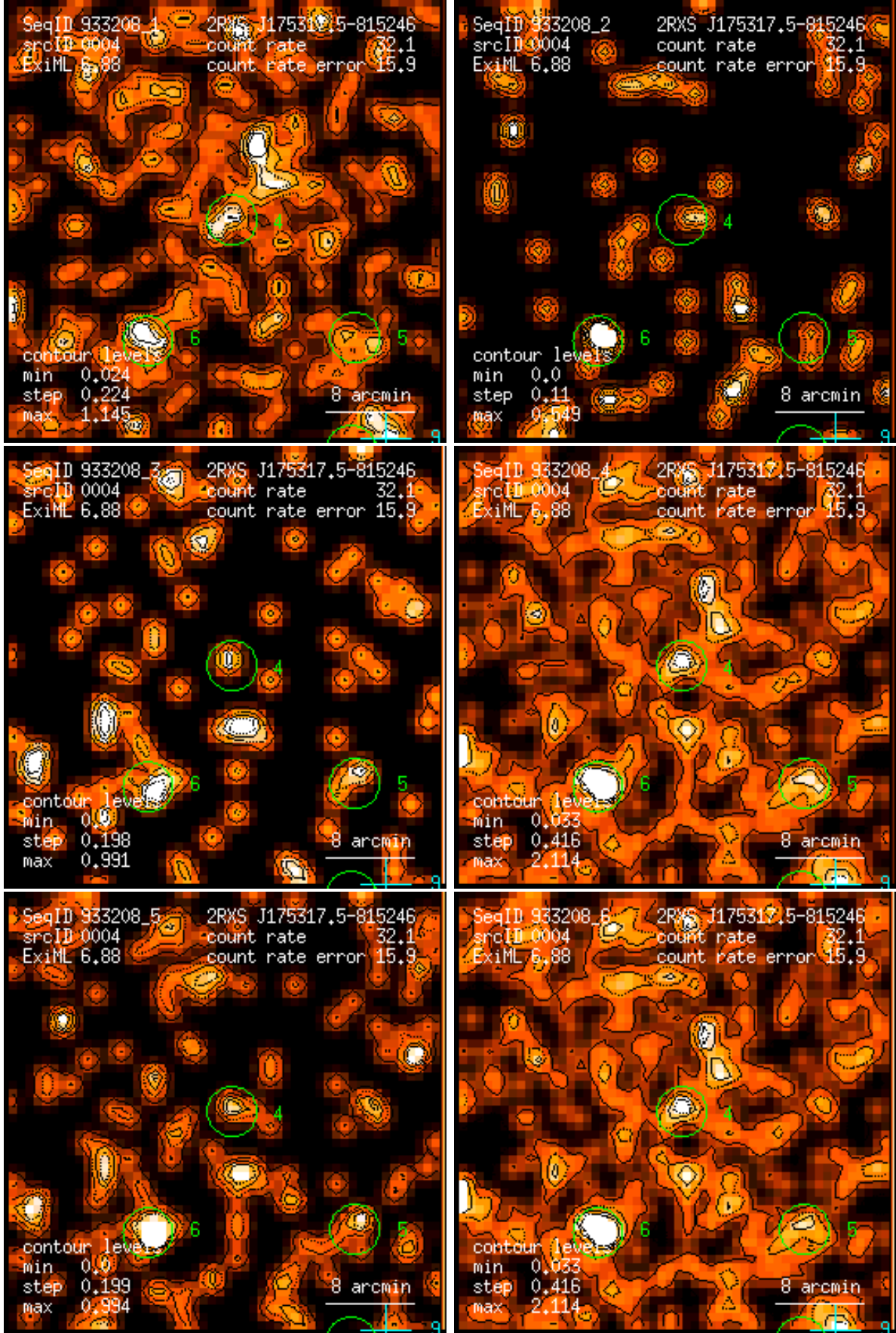
Figure 4: RASS 933208: detection 0004: band rate images, Gaussian filter: (1) PSPC channels 11 – 41, (2) 52 – 90, (3) 91 – 201, (4) 11 – 235, (5) 52 – 201, (6) 11 – 201. Broad band rates in counts/ks. Band rate contour levels in counts/ks/arcmin 2 .
