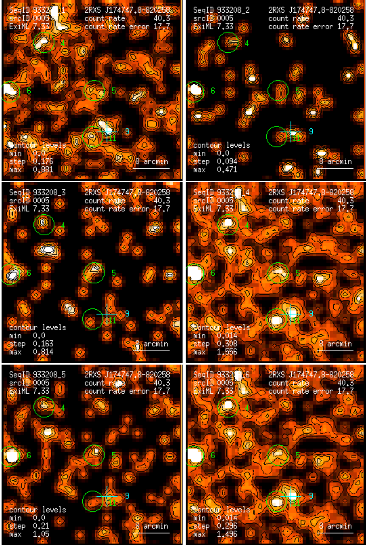
Figure 5: RASS 933208: detection 0005: band rate images, Gaussian filter: (1) PSPC channels 11 – 41, (2) 52 – 90, (3) 91 – 201, (4) 11 – 235, (5) 52 – 201, (6) 11 – 201. Broad band rates in counts/ks. Band rate contour levels in counts/ks/arcmin 2 .
