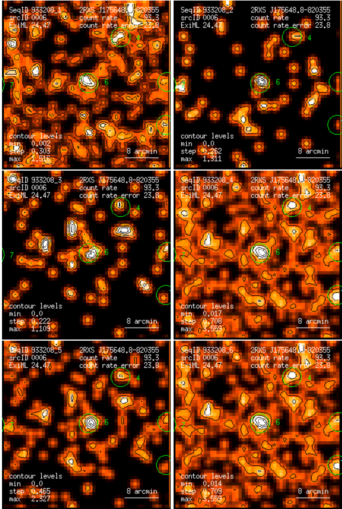
Figure 6: RASS 933208: detection 0006: band rate images, Gaussian filter: (1) PSPC channels 11 – 41, (2) 52 – 90, (3) 91 – 201, (4) 11 – 235, (5) 52 – 201, (6) 11 – 201. Broad band rates in counts/ks. Band rate contour levels in counts/ks/arcmin 2 .
