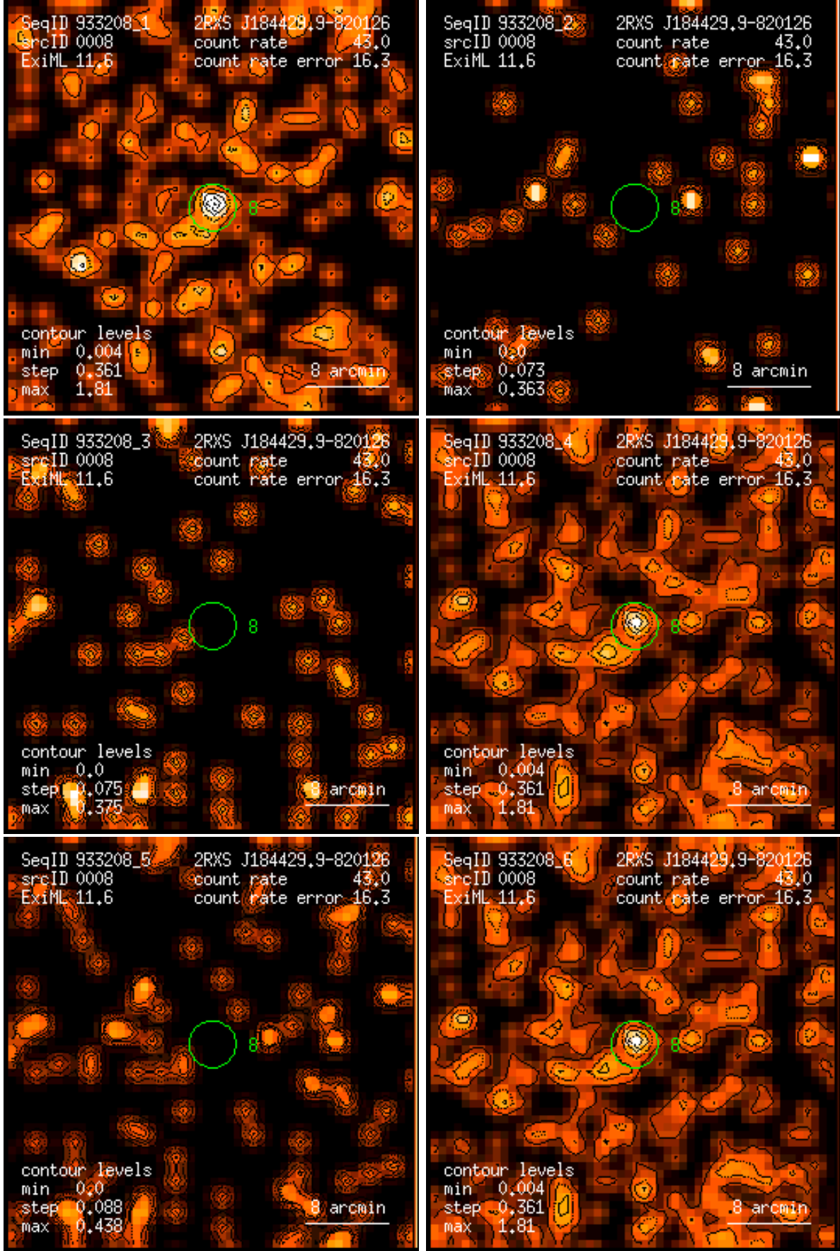
Figure 8: RASS 933208: detection 0008: band rate images, Gaussian filter: (1) PSPC channels 11 – 41, (2) 52 – 90, (3) 91 – 201, (4) 11 – 235, (5) 52 – 201, (6) 11 – 201. Broad band rates in counts/ks. Band rate contour levels in counts/ks/arcmin 2 .
