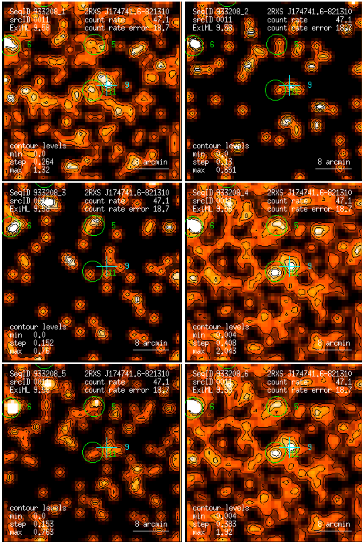
Figure 11: RASS 933208: detection 0011: band rate images, Gaussian filter: (1) PSPC channels 11 – 41, (2) 52 – 90, (3) 91 – 201, (4) 11 – 235, (5) 52 – 201, (6) 11 – 201. Broad band rates in counts/ks. Band rate contour levels in counts/ks/arcmin 2 .
