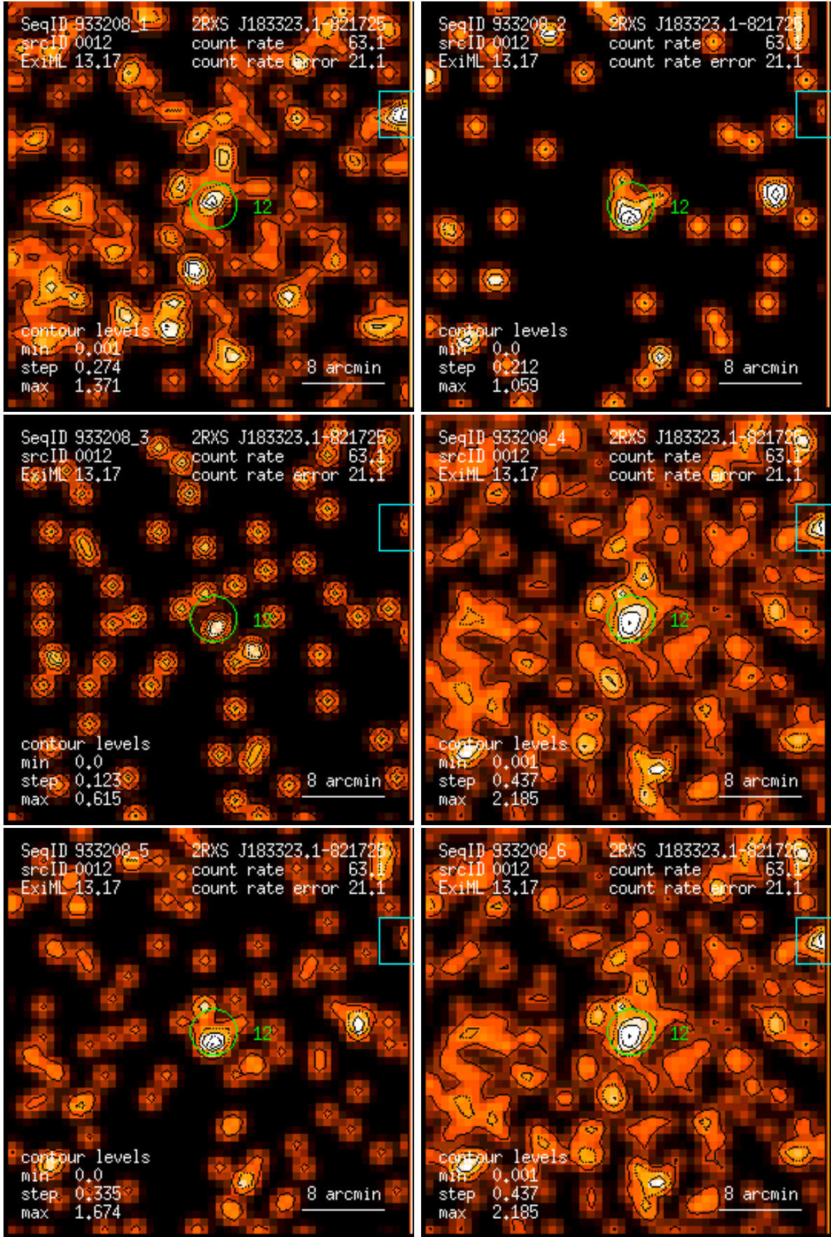
Figure 12: RASS 933208: detection 0012: band rate images, Gaussian filter: (1) PSPC channels 11 – 41, (2) 52 – 90, (3) 91 – 201, (4) 11 – 235, (5) 52 – 201, (6) 11 – 201. Broad band rates in counts/ks. Band rate contour levels in counts/ks/arcmin 2 .
