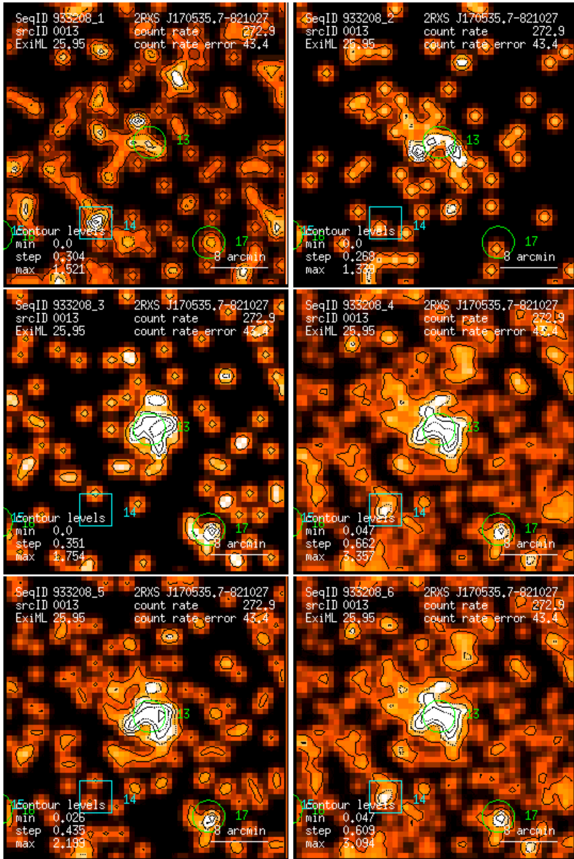
Figure 13: RASS 933208: detection 0013: band rate images, Gaussian filter: (1) PSPC channels 11 – 41, (2) 52 – 90, (3) 91 – 201, (4) 11 – 235, (5) 52 – 201, (6) 11 – 201. Broad band rates in counts/ks. Band rate contour levels in counts/ks/arcmin 2 .
