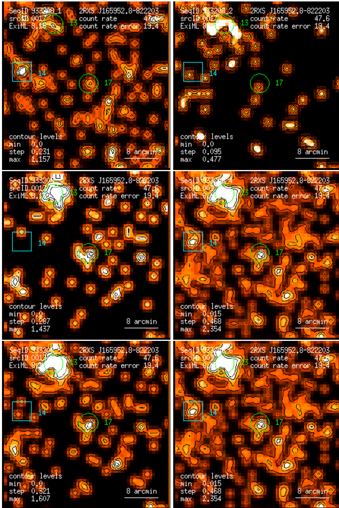
Figure 17: RASS 933208: detection 0017: band rate images, Gaussian filter: (1) PSPC channels 11 – 41, (2) 52 – 90, (3) 91 – 201, (4) 11 – 235, (5) 52 – 201, (6) 11 – 201. Broad band rates in counts/ks. Band rate contour levels in counts/ks/arcmin 2 .
