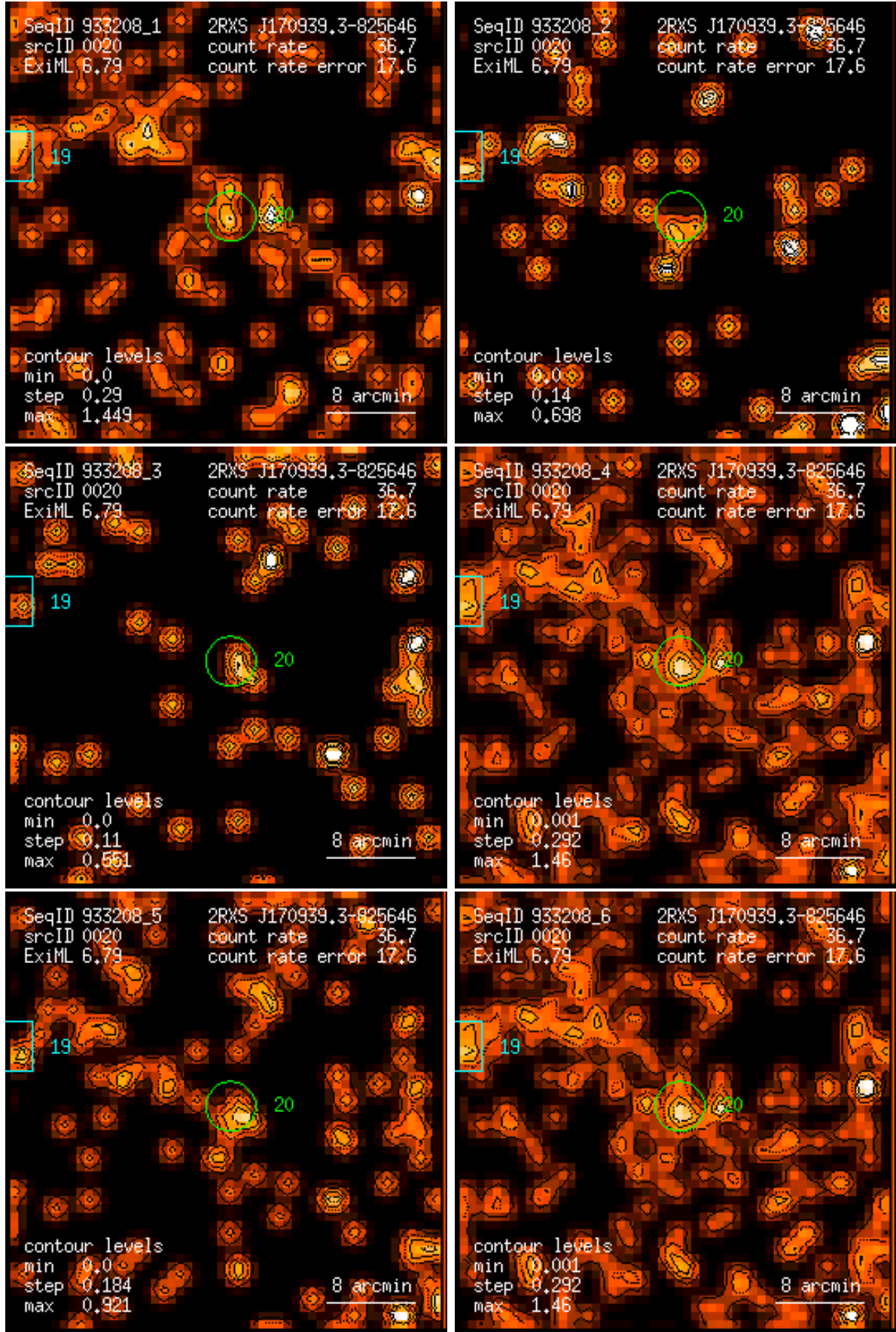
Figure 20: RASS 933208: detection 0020: band rate images, Gaussian filter: (1) PSPC channels 11 – 41, (2) 52 – 90, (3) 91 – 201, (4) 11 – 235, (5) 52 – 201, (6) 11 – 201. Broad band rates in counts/ks. Band rate contour levels in counts/ks/arcmin 2 .
