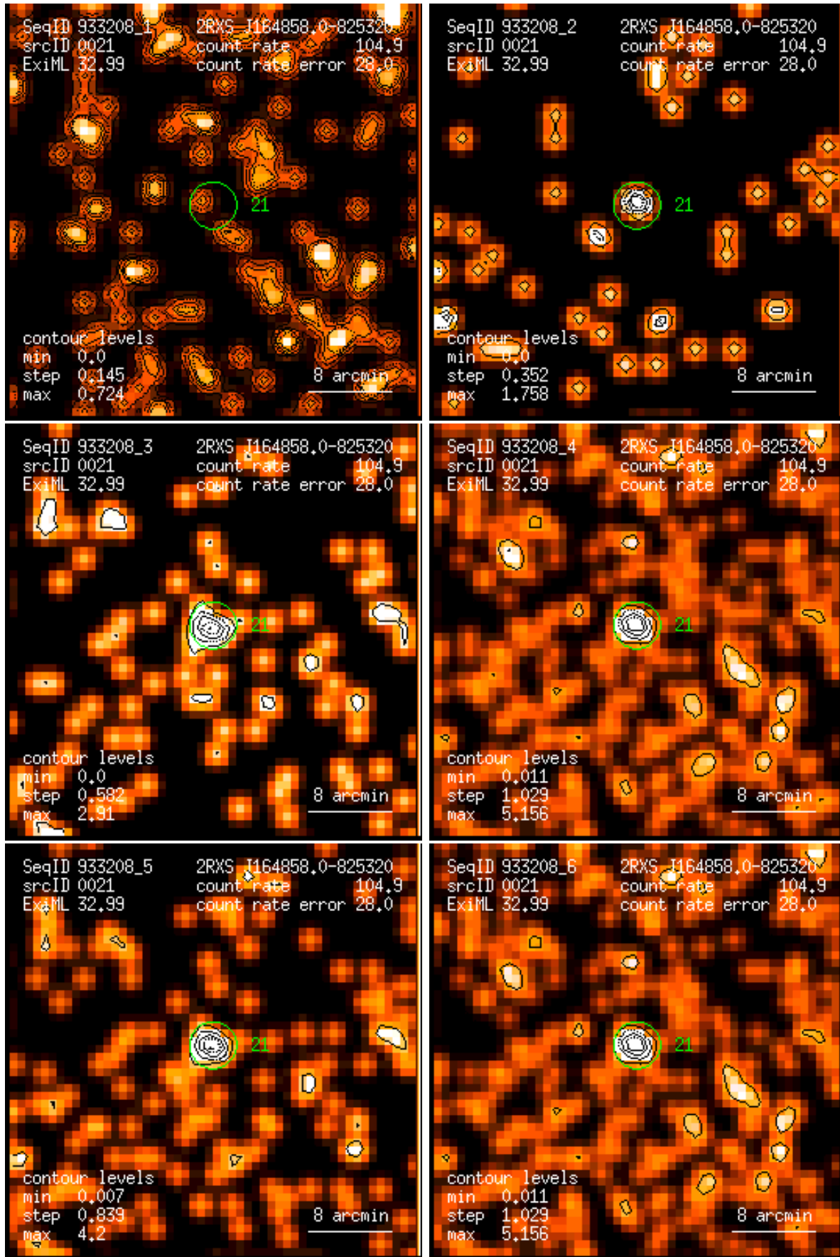
Figure 21: RASS 933208: detection 0021: band rate images, Gaussian filter: (1) PSPC channels 11 – 41, (2) 52 – 90, (3) 91 – 201, (4) 11 – 235, (5) 52 – 201, (6) 11 – 201. Broad band rates in counts/ks. Band rate contour levels in counts/ks/arcmin 2 .
