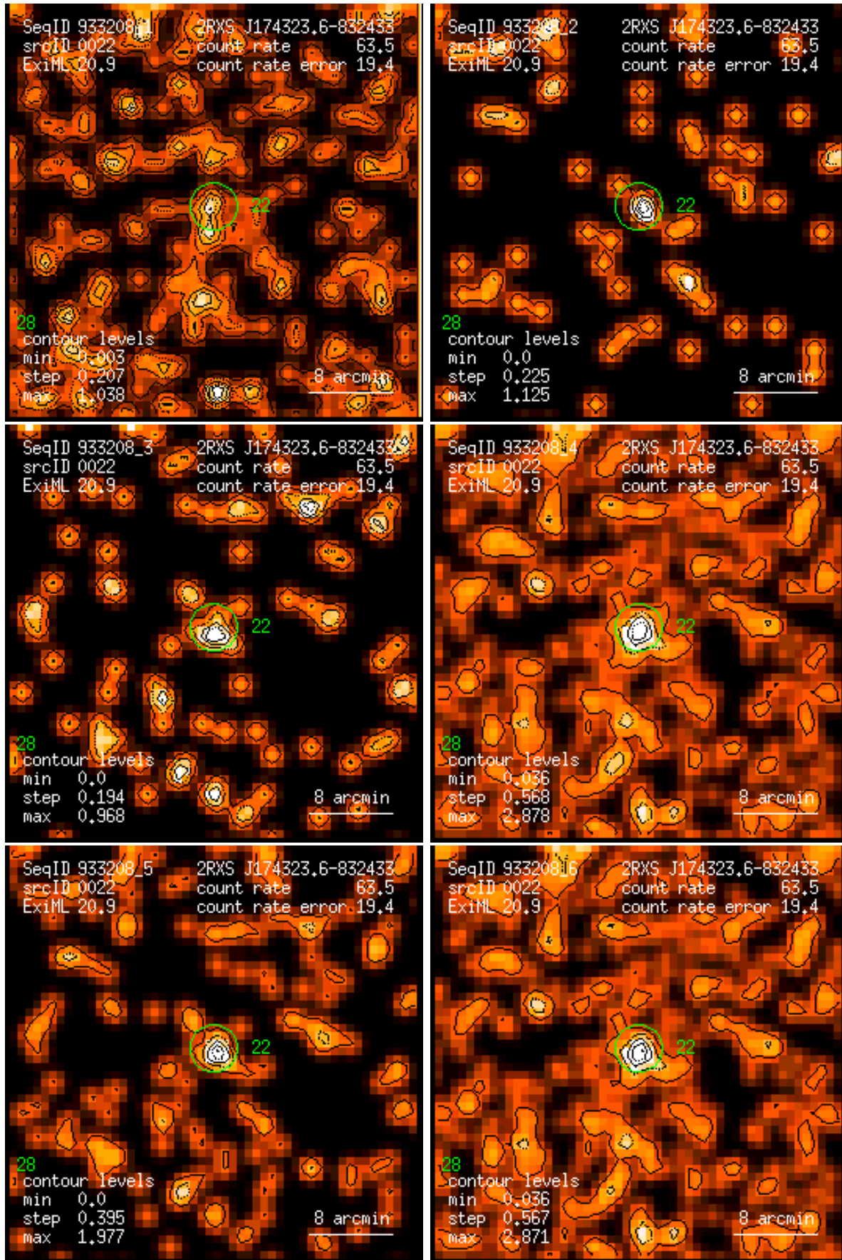
Figure 22: RASS 933208: detection 0022: band rate images, Gaussian filter: (1) PSPC channels 11 – 41, (2) 52 – 90, (3) 91 – 201, (4) 11 – 235, (5) 52 – 201, (6) 11 – 201. Broad band rates in counts/ks. Band rate contour levels in counts/ks/arcmin 2 .
