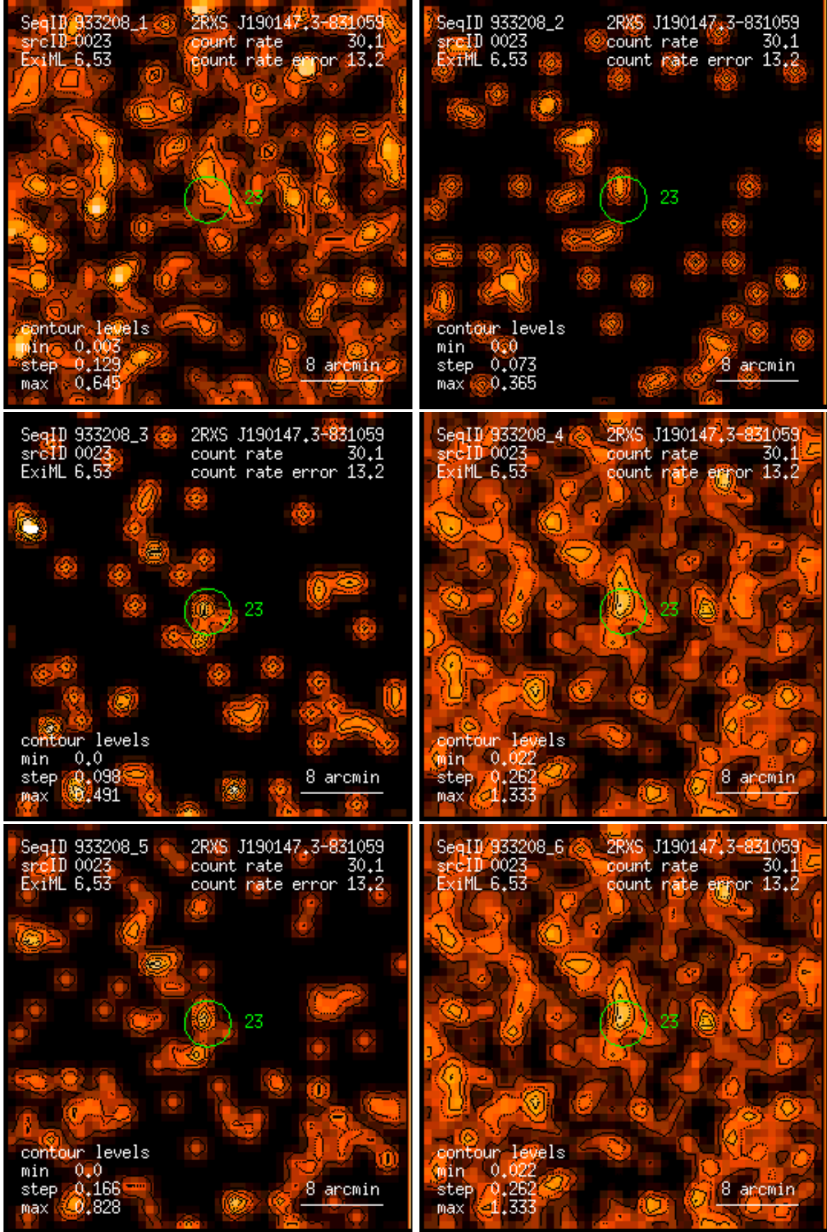
Figure 23: RASS 933208: detection 0023: band rate images, Gaussian filter: (1) PSPC channels 11 – 41, (2) 52 – 90, (3) 91 – 201, (4) 11 – 235, (5) 52 – 201, (6) 11 – 201. Broad band rates in counts/ks. Band rate contour levels in counts/ks/arcmin 2 .
