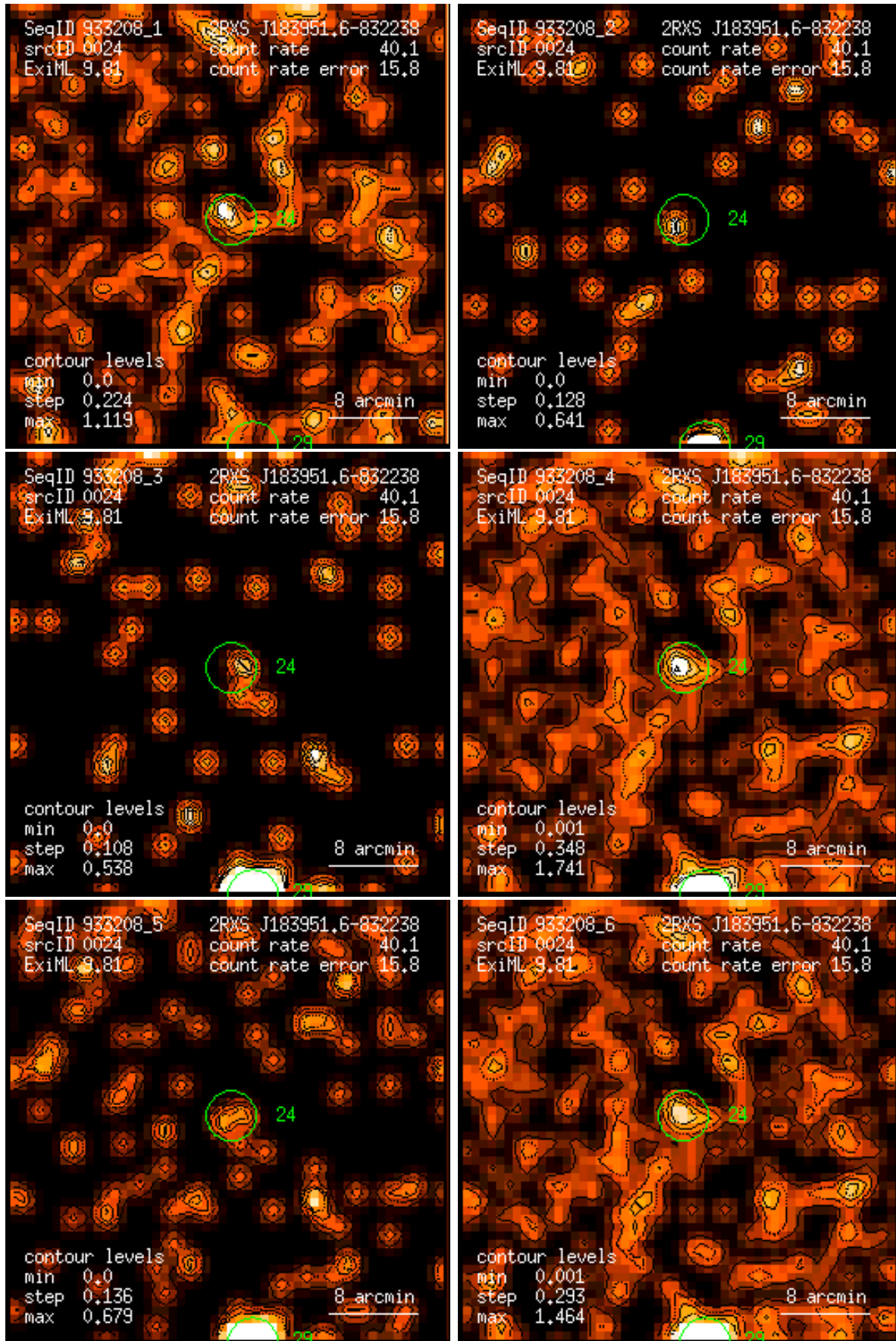
Figure 24: RASS 933208: detection 0024: band rate images, Gaussian filter: (1) PSPC channels 11 – 41, (2) 52 – 90, (3) 91 – 201, (4) 11 – 235, (5) 52 – 201, (6) 11 – 201. Broad band rates in counts/ks. Band rate contour levels in counts/ks/arcmin 2 .
