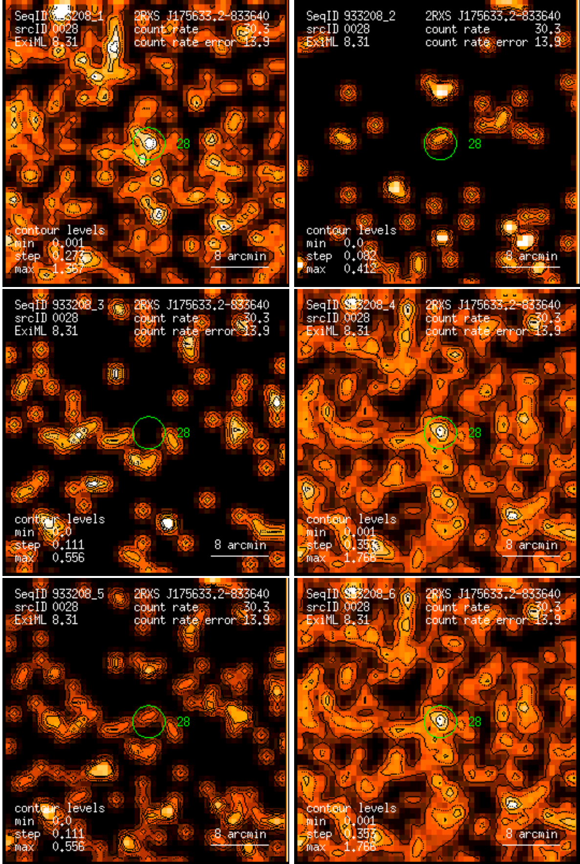
Figure 28: RASS 933208: detection 0028: band rate images, Gaussian filter: (1) PSPC channels 11 – 41, (2) 52 – 90, (3) 91 – 201, (4) 11 – 235, (5) 52 – 201, (6) 11 – 201. Broad band rates in counts/ks. Band rate contour levels in counts/ks/arcmin 2 .
