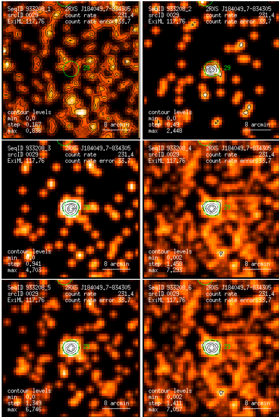
Figure 29: RASS 933208: detection 0029: band rate images, Gaussian filter: (1) PSPC channels 11 – 41, (2) 52 – 90, (3) 91 – 201, (4) 11 – 235, (5) 52 – 201, (6) 11 – 201. Broad band rates in counts/ks. Band rate contour levels in counts/ks/arcmin 2 .
