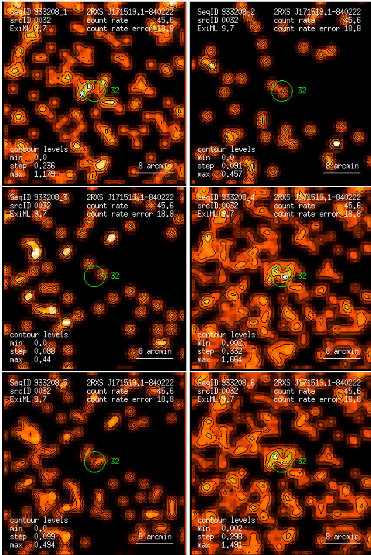
Figure 32: RASS 933208: detection 0032: band rate images, Gaussian filter: (1) PSPC channels 11 – 41, (2) 52 – 90, (3) 91 – 201, (4) 11 – 235, (5) 52 – 201, (6) 11 – 201. Broad band rates in counts/ks. Band rate contour levels in counts/ks/arcmin 2 .
