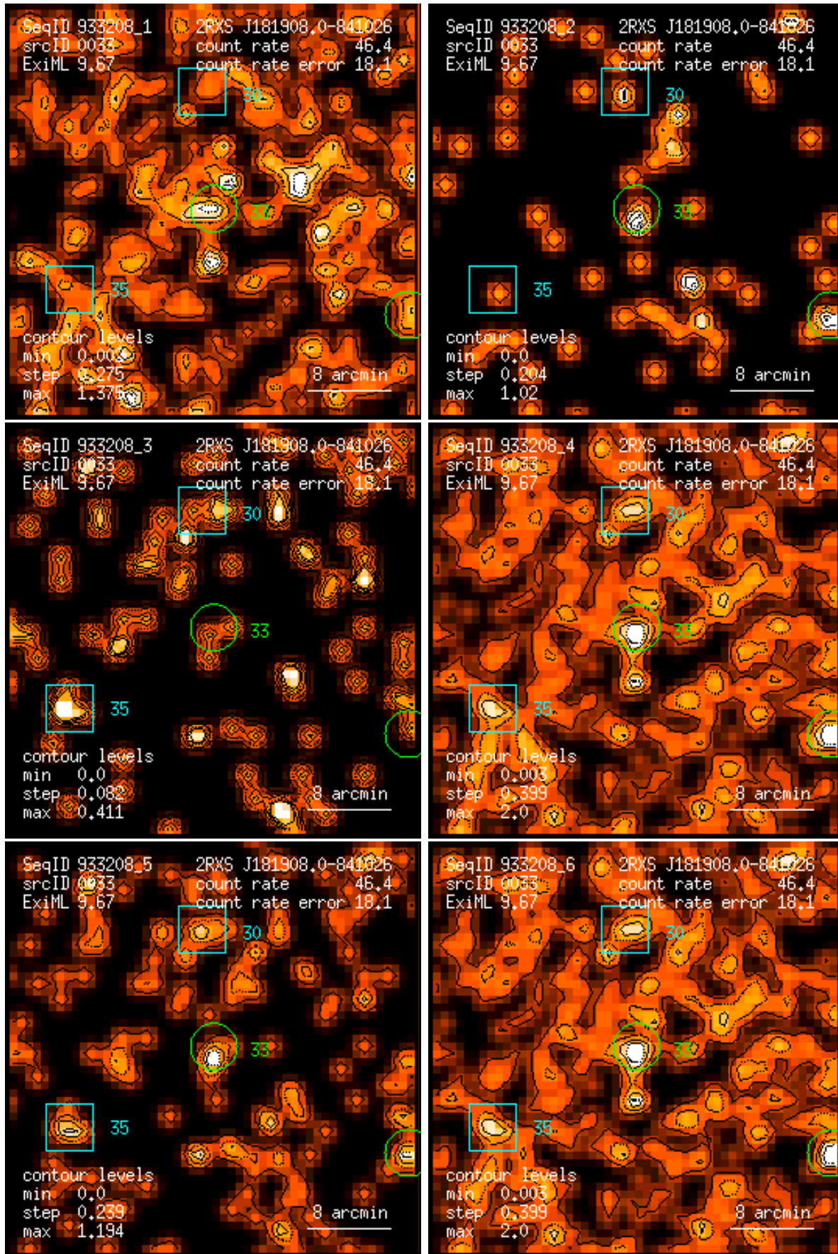
Figure 33: RASS 933208: detection 0033: band rate images, Gaussian filter: (1) PSPC channels 11 – 41, (2) 52 – 90, (3) 91 – 201, (4) 11 – 235, (5) 52 – 201, (6) 11 – 201. Broad band rates in counts/ks. Band rate contour levels in counts/ks/arcmin 2 .
