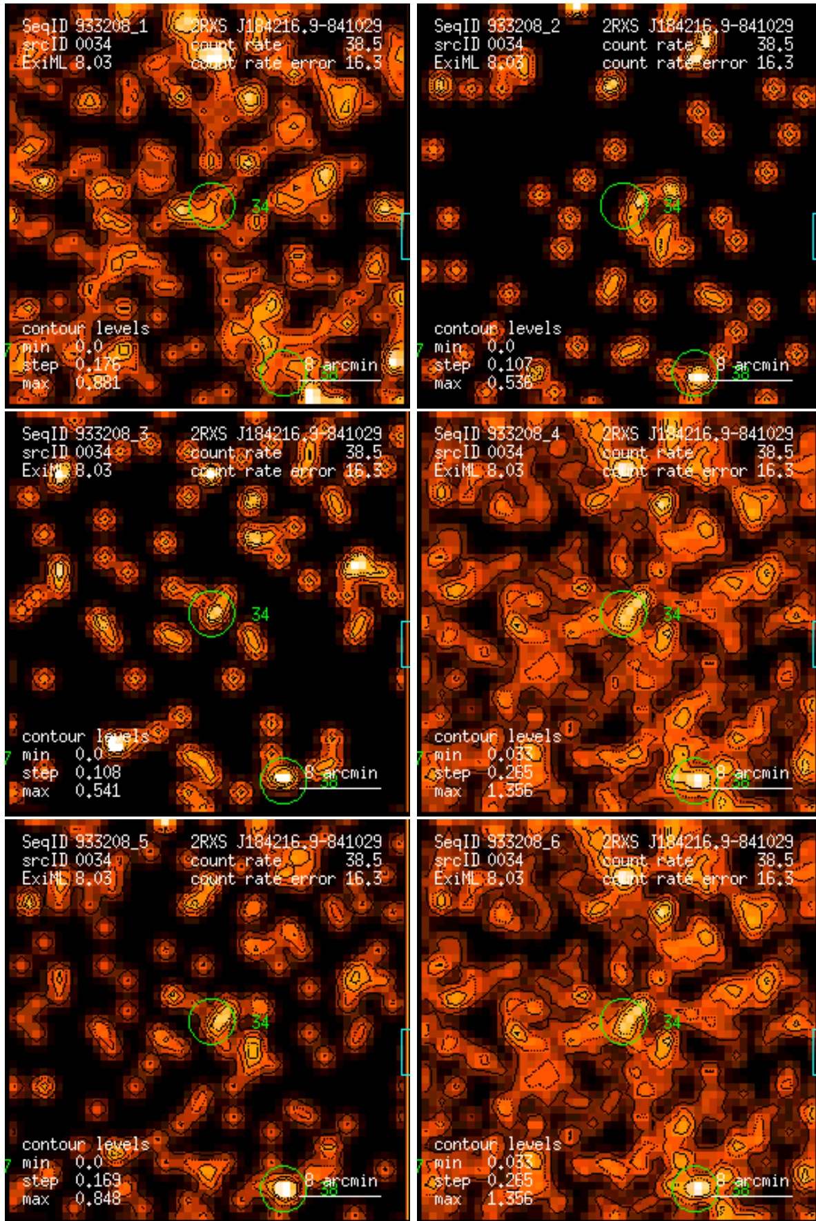
Figure 34: RASS 933208: detection 0034: band rate images, Gaussian filter: (1) PSPC channels 11 – 41, (2) 52 – 90, (3) 91 – 201, (4) 11 – 235, (5) 52 – 201, (6) 11 – 201. Broad band rates in counts/ks. Band rate contour levels in counts/ks/arcmin 2 .
