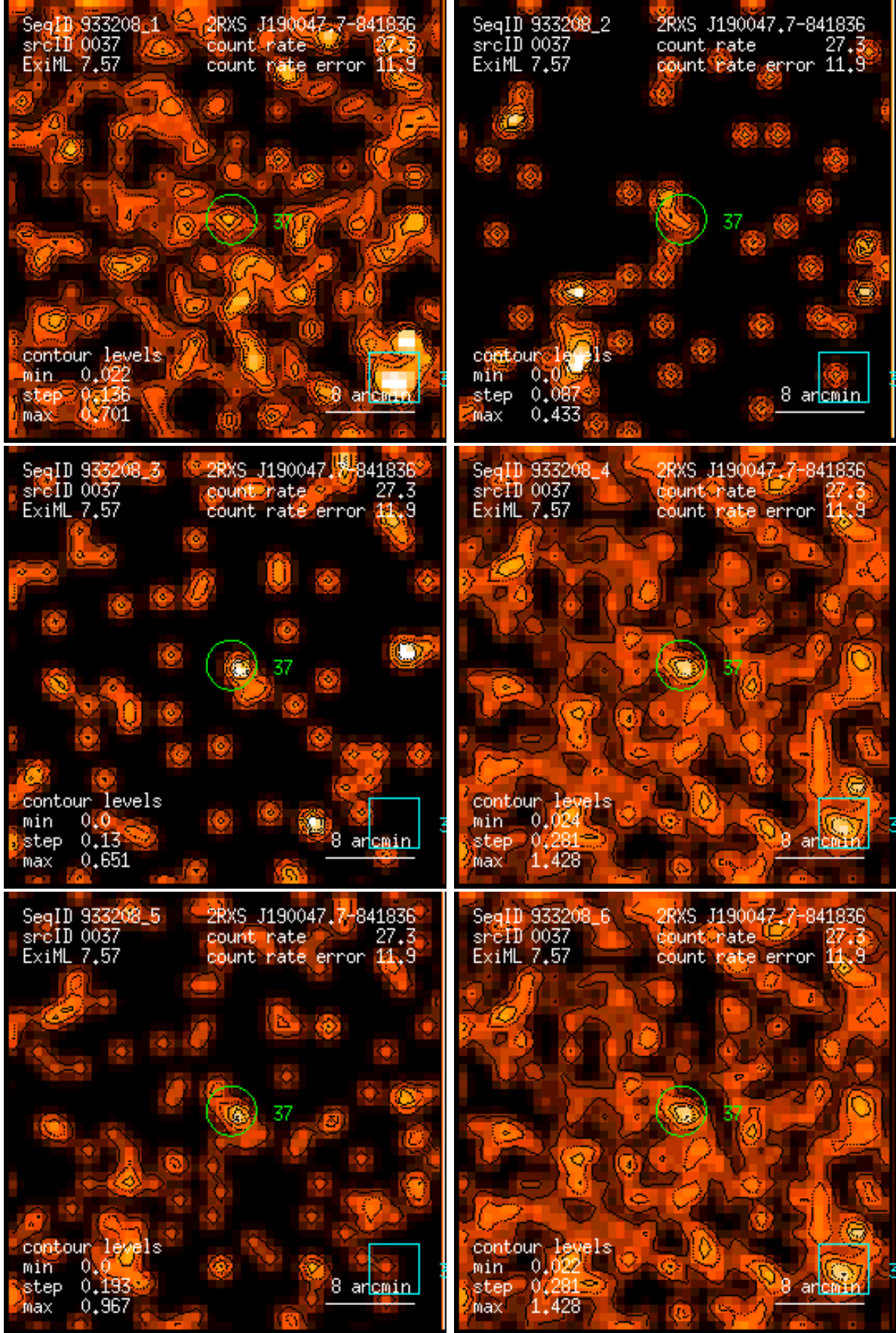
Figure 37: RASS 933208: detection 0037: band rate images, Gaussian filter: (1) PSPC channels 11 – 41, (2) 52 – 90, (3) 91 – 201, (4) 11 – 235, (5) 52 – 201, (6) 11 – 201. Broad band rates in counts/ks. Band rate contour levels in counts/ks/arcmin 2 .
