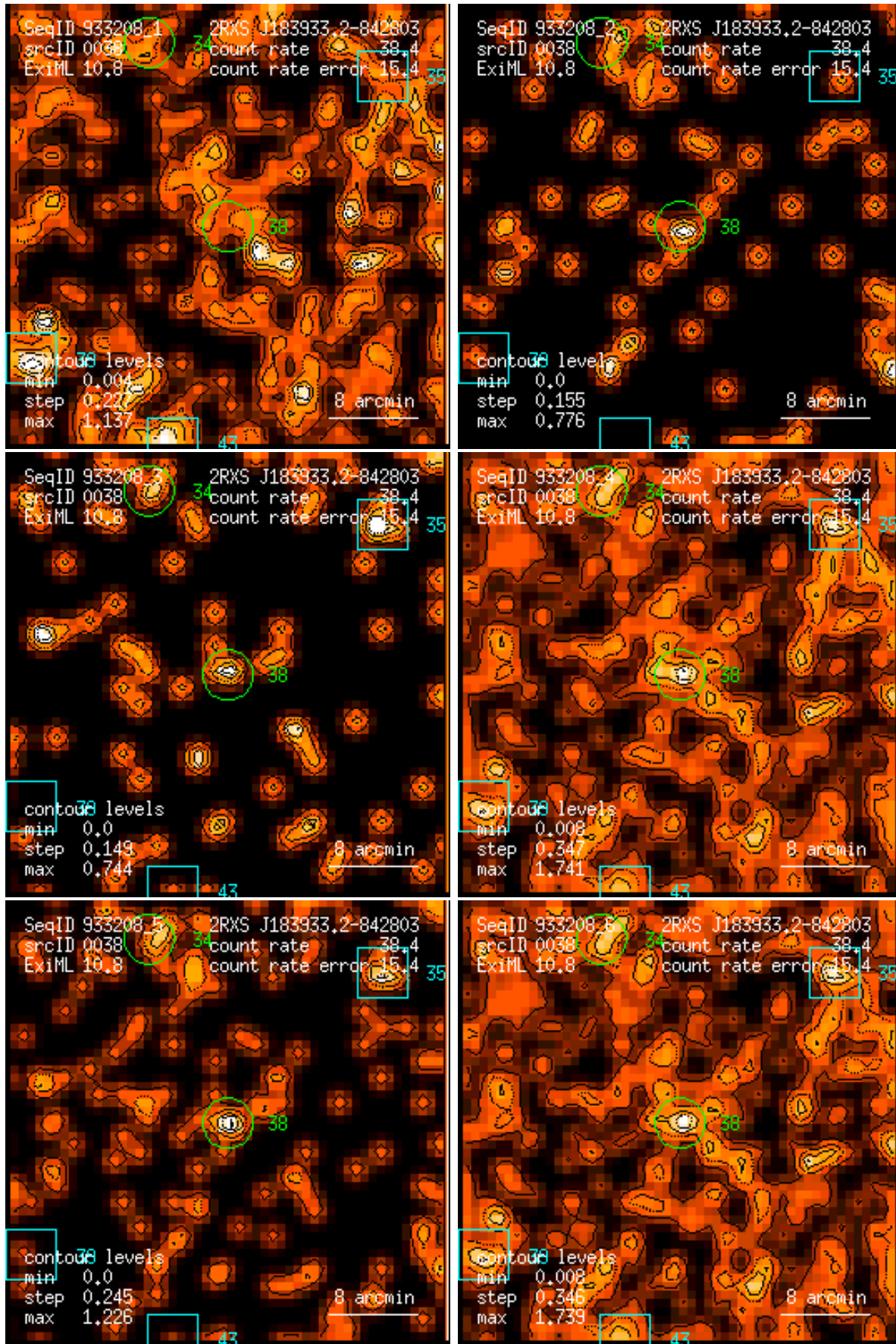
Figure 38: RASS 933208: detection 0038: band rate images, Gaussian filter: (1) PSPC channels 11 – 41, (2) 52 – 90, (3) 91 – 201, (4) 11 – 235, (5) 52 – 201, (6) 11 – 201. Broad band rates in counts/ks. Band rate contour levels in counts/ks/arcmin 2 .
