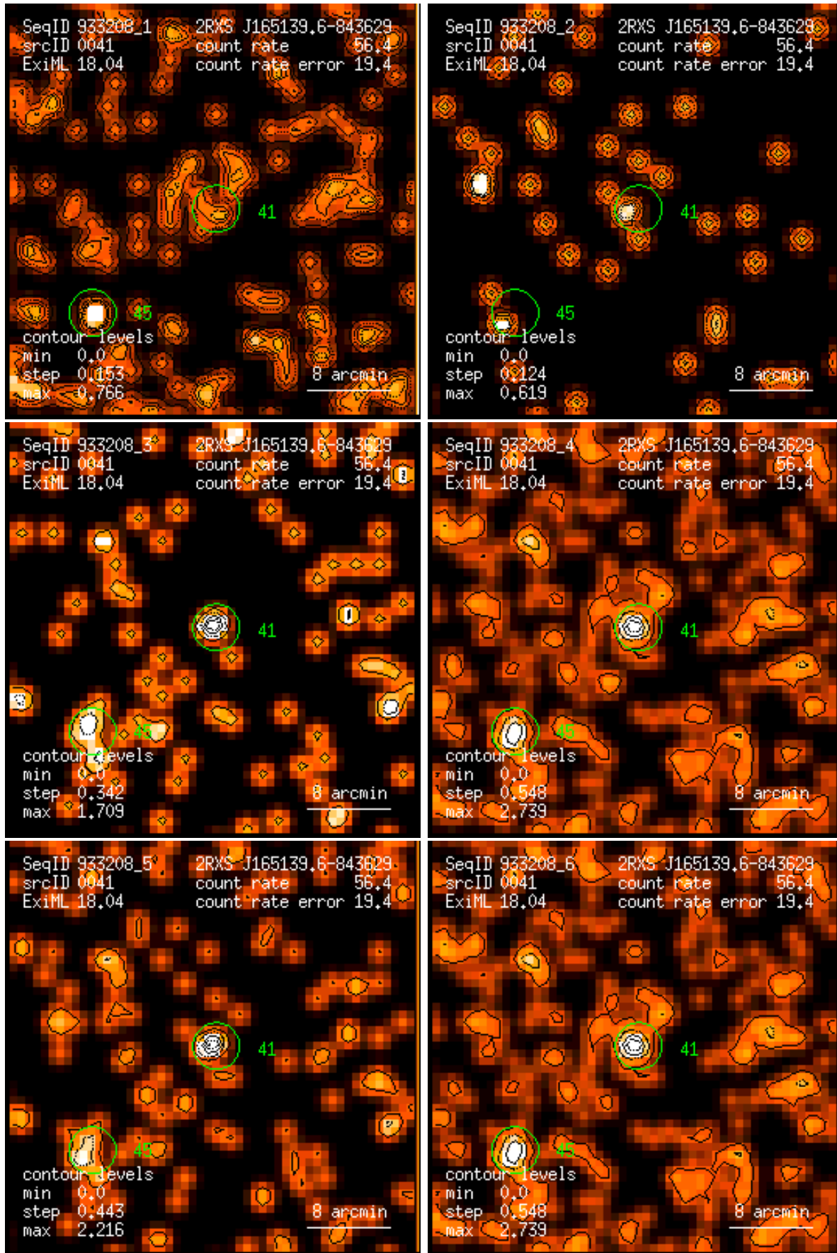
Figure 41: RASS 933208: detection 0041: band rate images, Gaussian filter: (1) PSPC channels 11 – 41, (2) 52 – 90, (3) 91 – 201, (4) 11 – 235, (5) 52 – 201, (6) 11 – 201. Broad band rates in counts/ks. Band rate contour levels in counts/ks/arcmin 2 .
