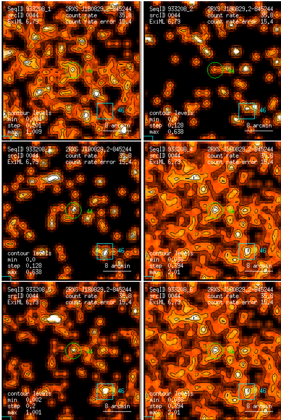
Figure 44: RASS 933208: detection 0044: band rate images, Gaussian filter: (1) PSPC channels 11 – 41, (2) 52 – 90, (3) 91 – 201, (4) 11 – 235, (5) 52 – 201, (6) 11 – 201. Broad band rates in counts/ks. Band rate contour levels in counts/ks/arcmin 2 .
