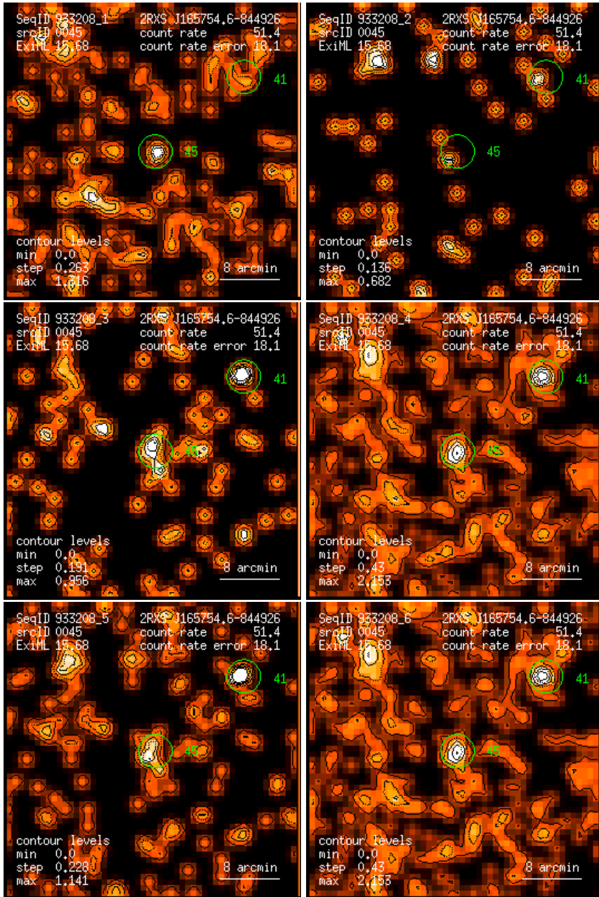
Figure 45: RASS 933208: detection 0045: band rate images, Gaussian filter: (1) PSPC channels 11 – 41, (2) 52 – 90, (3) 91 – 201, (4) 11 – 235, (5) 52 – 201, (6) 11 – 201. Broad band rates in counts/ks. Band rate contour levels in counts/ks/arcmin 2 .
