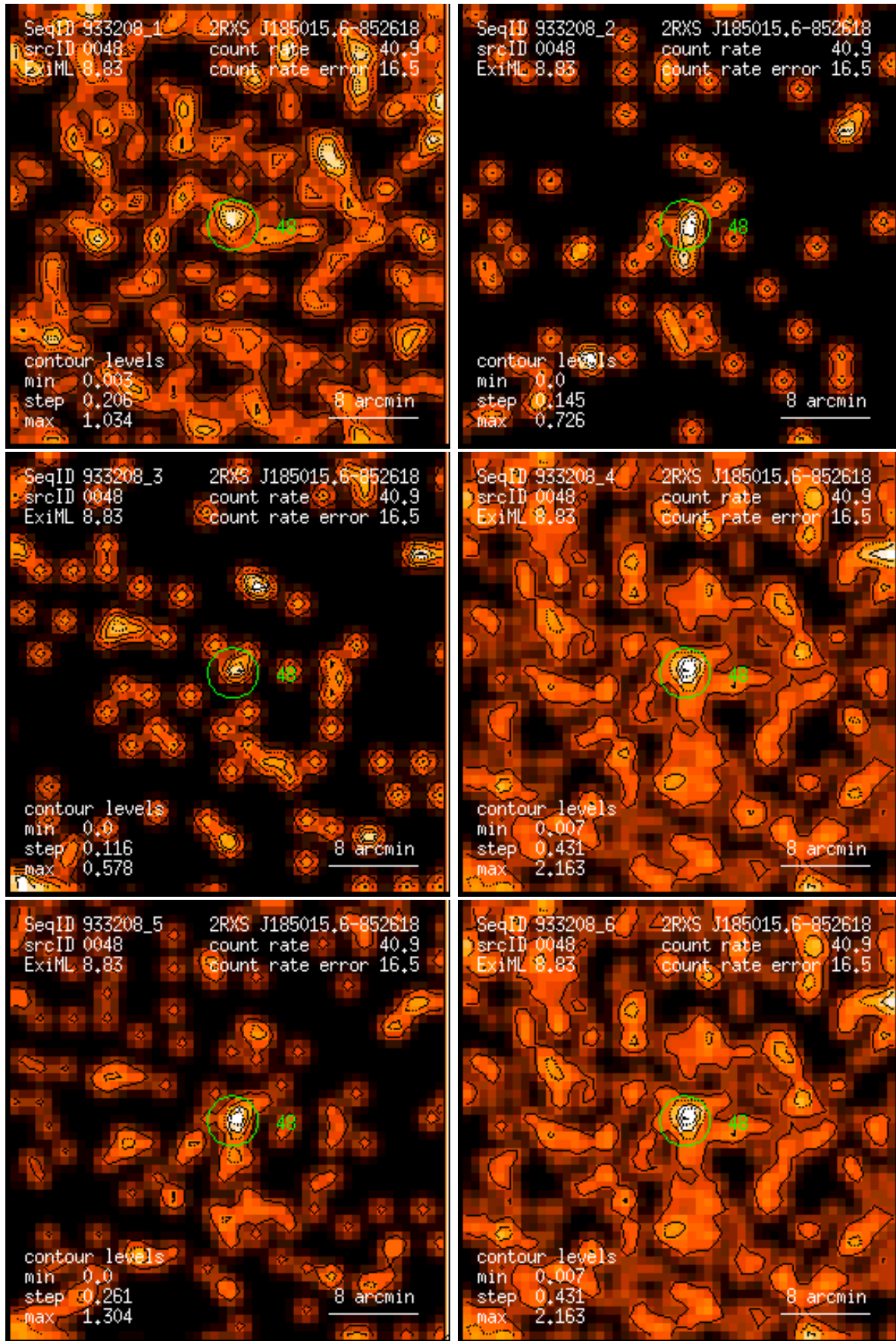
Figure 48: RASS 933208: detection 0048: band rate images, Gaussian filter: (1) PSPC channels 11 – 41, (2) 52 – 90, (3) 91 – 201, (4) 11 – 235, (5) 52 – 201, (6) 11 – 201. Broad band rates in counts/ks. Band rate contour levels in counts/ks/arcmin 2 .
