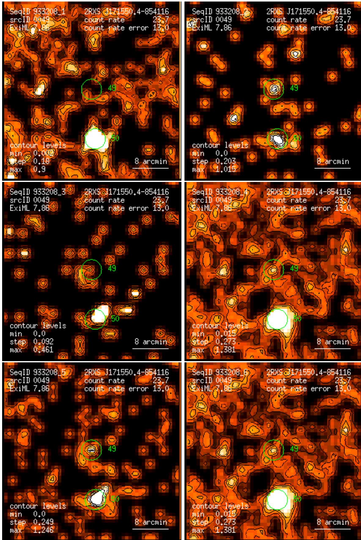
Figure 49: RASS 933208: detection 0049: band rate images, Gaussian filter: (1) PSPC channels 11 – 41, (2) 52 – 90, (3) 91 – 201, (4) 11 – 235, (5) 52 – 201, (6) 11 – 201. Broad band rates in counts/ks. Band rate contour levels in counts/ks/arcmin 2 .
