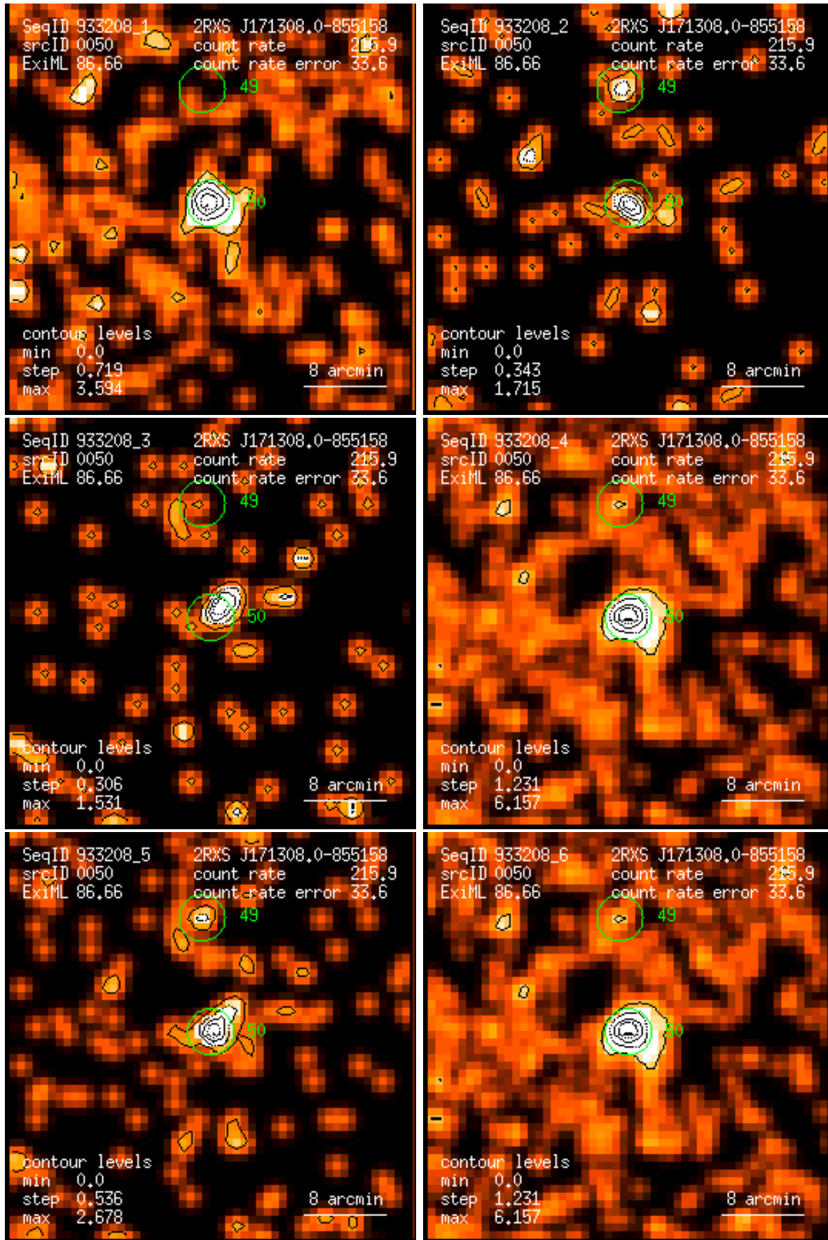
Figure 50: RASS 933208: detection 0050: band rate images, Gaussian filter: (1) PSPC channels 11 – 41, (2) 52 – 90, (3) 91 – 201, (4) 11 – 235, (5) 52 – 201, (6) 11 – 201. Broad band rates in counts/ks. Band rate contour levels in counts/ks/arcmin 2 .
