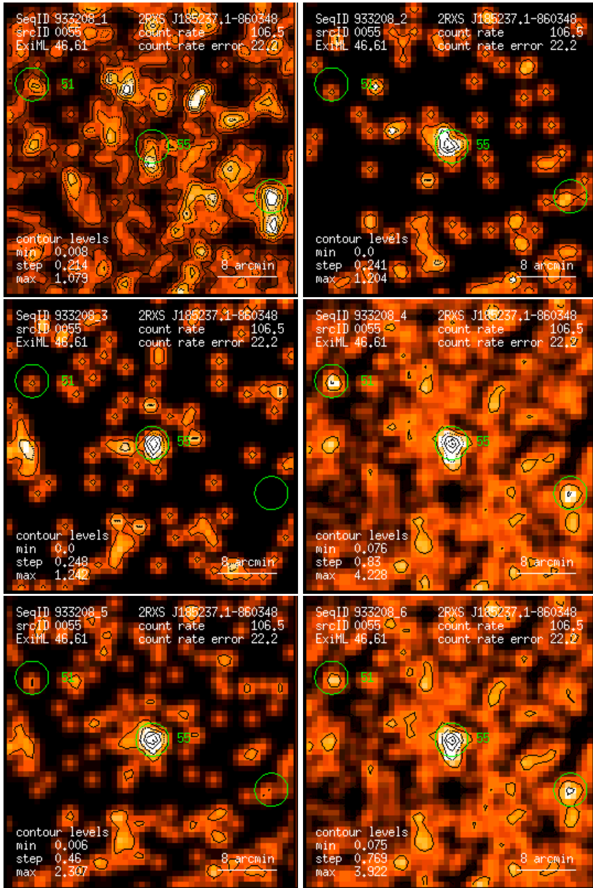
Figure 55: RASS 933208: detection 0055: band rate images, Gaussian filter: (1) PSPC channels 11 – 41, (2) 52 – 90, (3) 91 – 201, (4) 11 – 235, (5) 52 – 201, (6) 11 – 201. Broad band rates in counts/ks. Band rate contour levels in counts/ks/arcmin 2 .
