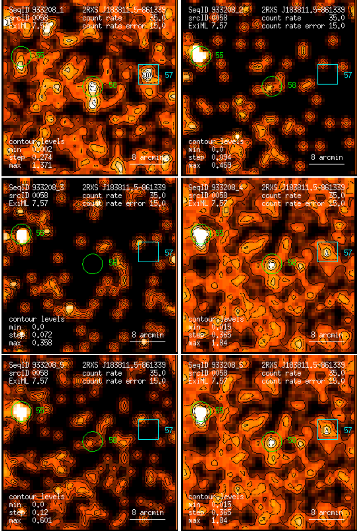
Figure 58: RASS 933208: detection 0058: band rate images, Gaussian filter: (1) PSPC channels 11 – 41, (2) 52 – 90, (3) 91 – 201, (4) 11 – 235, (5) 52 – 201, (6) 11 – 201. Broad band rates in counts/ks. Band rate contour levels in counts/ks/arcmin 2 .
