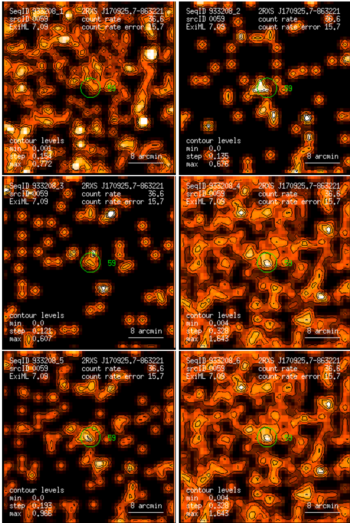
Figure 59: RASS 933208: detection 0059: band rate images, Gaussian filter: (1) PSPC channels 11 – 41, (2) 52 – 90, (3) 91 – 201, (4) 11 – 235, (5) 52 – 201, (6) 11 – 201. Broad band rates in counts/ks. Band rate contour levels in counts/ks/arcmin 2 .
