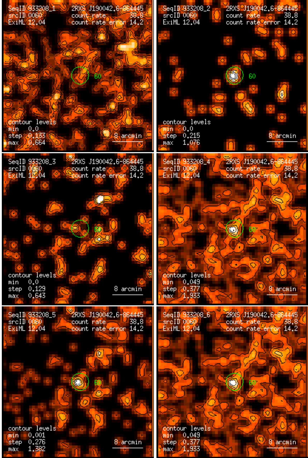
Figure 60: RASS 933208: detection 0060: band rate images, Gaussian filter: (1) PSPC channels 11 – 41, (2) 52 – 90, (3) 91 – 201, (4) 11 – 235, (5) 52 – 201, (6) 11 – 201. Broad band rates in counts/ks. Band rate contour levels in counts/ks/arcmin 2 .
