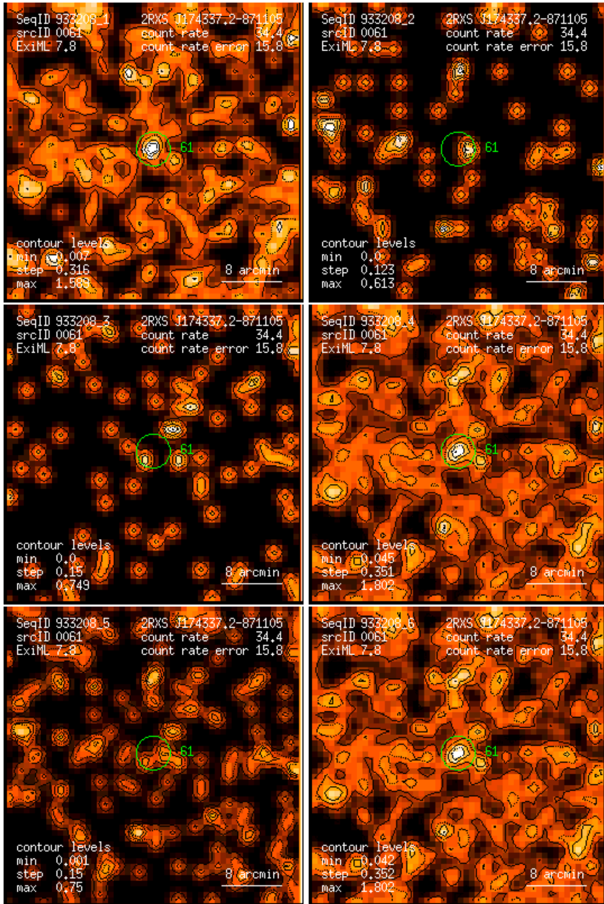
Figure 61: RASS 933208: detection 0061: band rate images, Gaussian filter: (1) PSPC channels 11 – 41, (2) 52 – 90, (3) 91 – 201, (4) 11 – 235, (5) 52 – 201, (6) 11 – 201. Broad band rates in counts/ks. Band rate contour levels in counts/ks/arcmin 2 .
