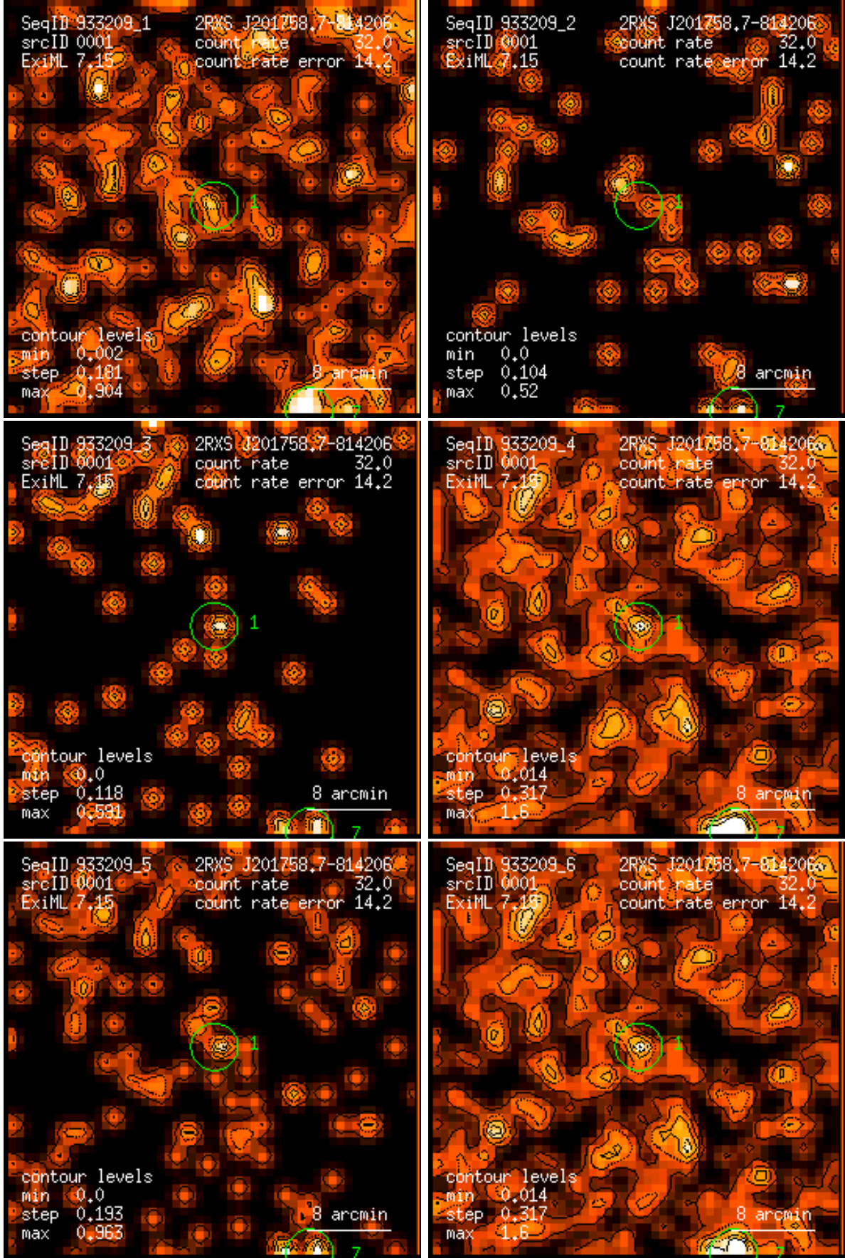
Figure 1: RASS 933209: detection 0001: band rate images, Gaussian filter: (1) PSPC channels 11 – 41, (2) 52 – 90, (3) 91 – 201, (4) 11 – 235, (5) 52 – 201, (6) 11 – 201. Broad band rates in counts/ks. Band rate contour levels in counts/ks/arcmin 2 .
