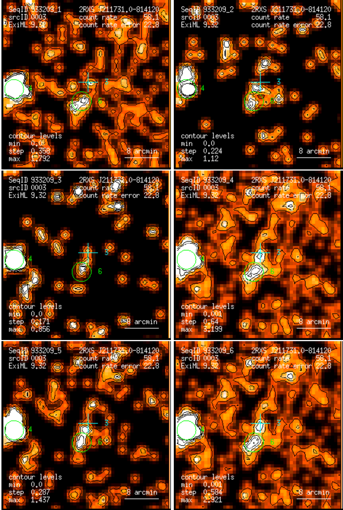
Figure 3: RASS 933209: detection 0003: band rate images, Gaussian filter: (1) PSPC channels 11 – 41, (2) 52 – 90, (3) 91 – 201, (4) 11 – 235, (5) 52 – 201, (6) 11 – 201. Broad band rates in counts/ks. Band rate contour levels in counts/ks/arcmin 2 .
