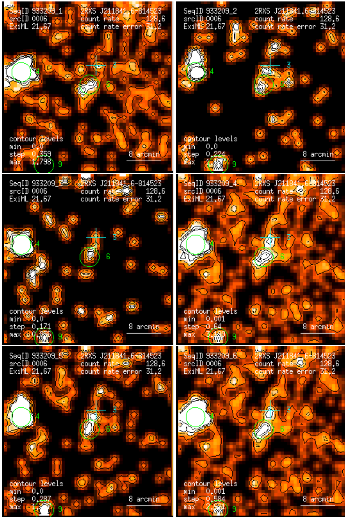
Figure 6: RASS 933209: detection 0006: band rate images, Gaussian filter: (1) PSPC channels 11 – 41, (2) 52 – 90, (3) 91 – 201, (4) 11 – 235, (5) 52 – 201, (6) 11 – 201. Broad band rates in counts/ks. Band rate contour levels in counts/ks/arcmin 2 .
